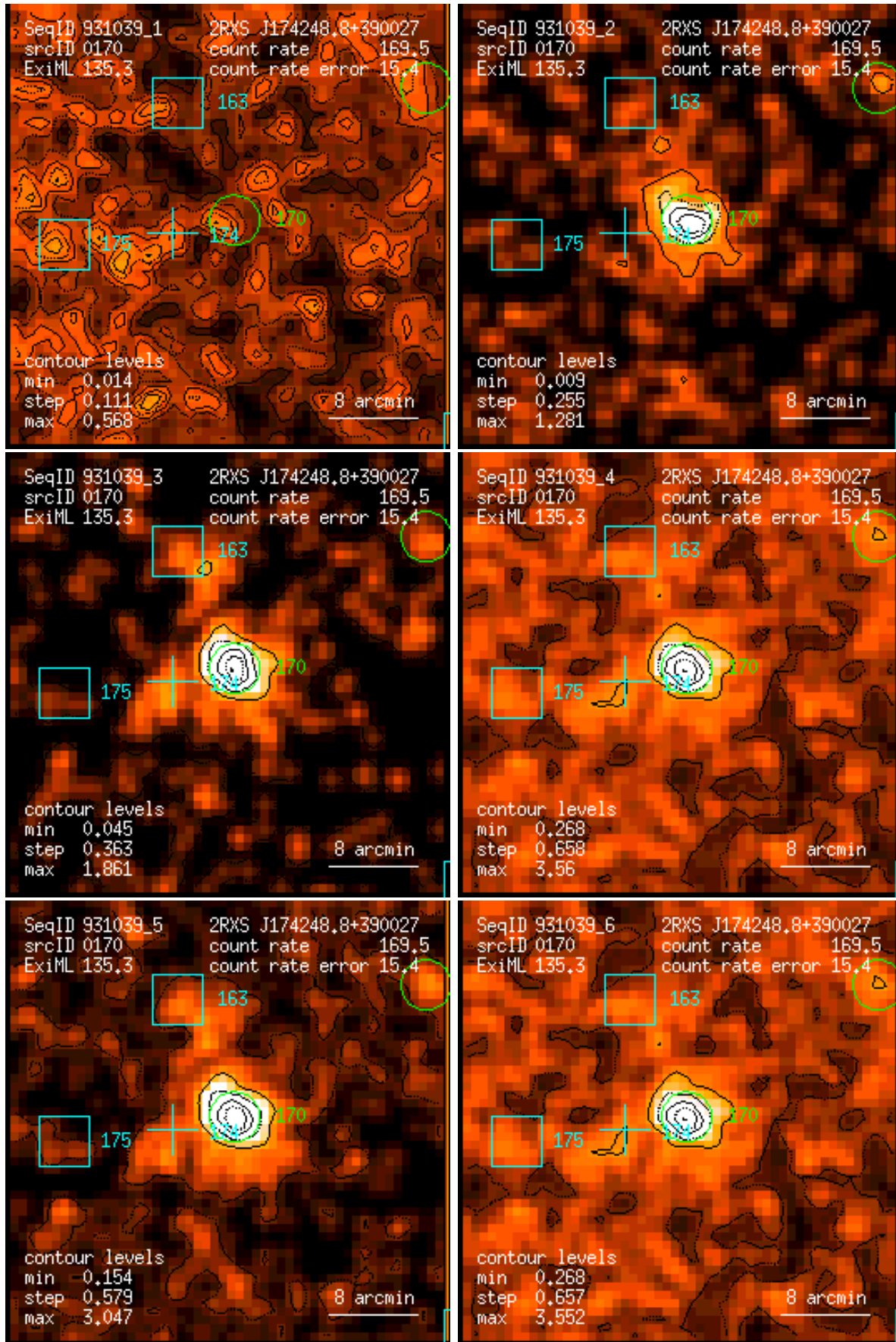
Figure 170: RASS 931039: detection 0170: band rate images, Gaussian filter: (1) PSPC channels 11 – 41, (2) 52 – 90, (3) 91 – 201, (4) 11 – 235, (5) 52 – 201, (6) 11 – 201. Broad band rates in counts/ks. Band rate contour levels in counts/ks/arcmin 2 .
