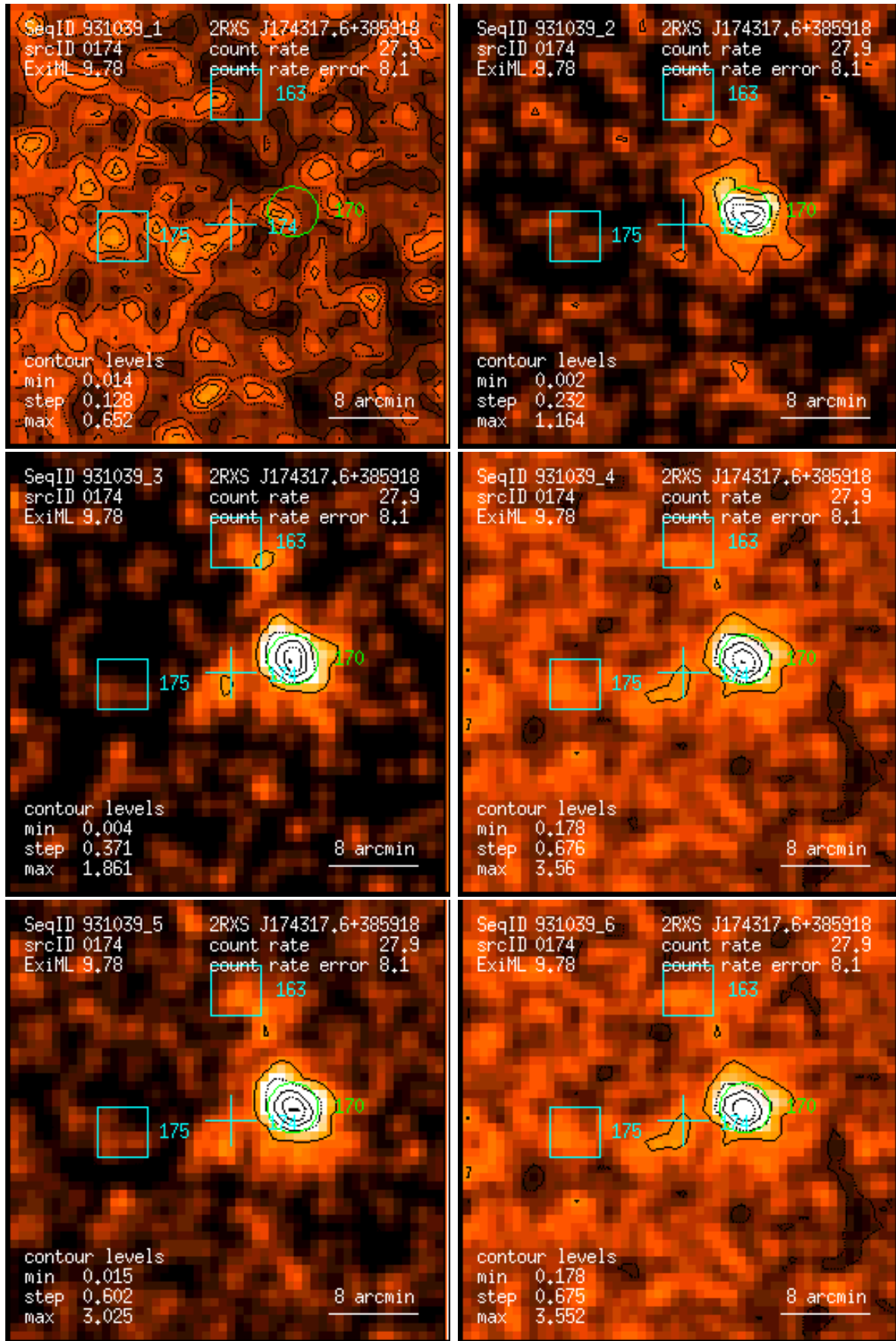
Figure 174: RASS 931039: detection 0174: band rate images, Gaussian filter: (1) PSPC channels 11 – 41, (2) 52 – 90, (3) 91 – 201, (4) 11 – 235, (5) 52 – 201, (6) 11 – 201. Broad band rates in counts/ks. Band rate contour levels in counts/ks/arcmin 2 .
