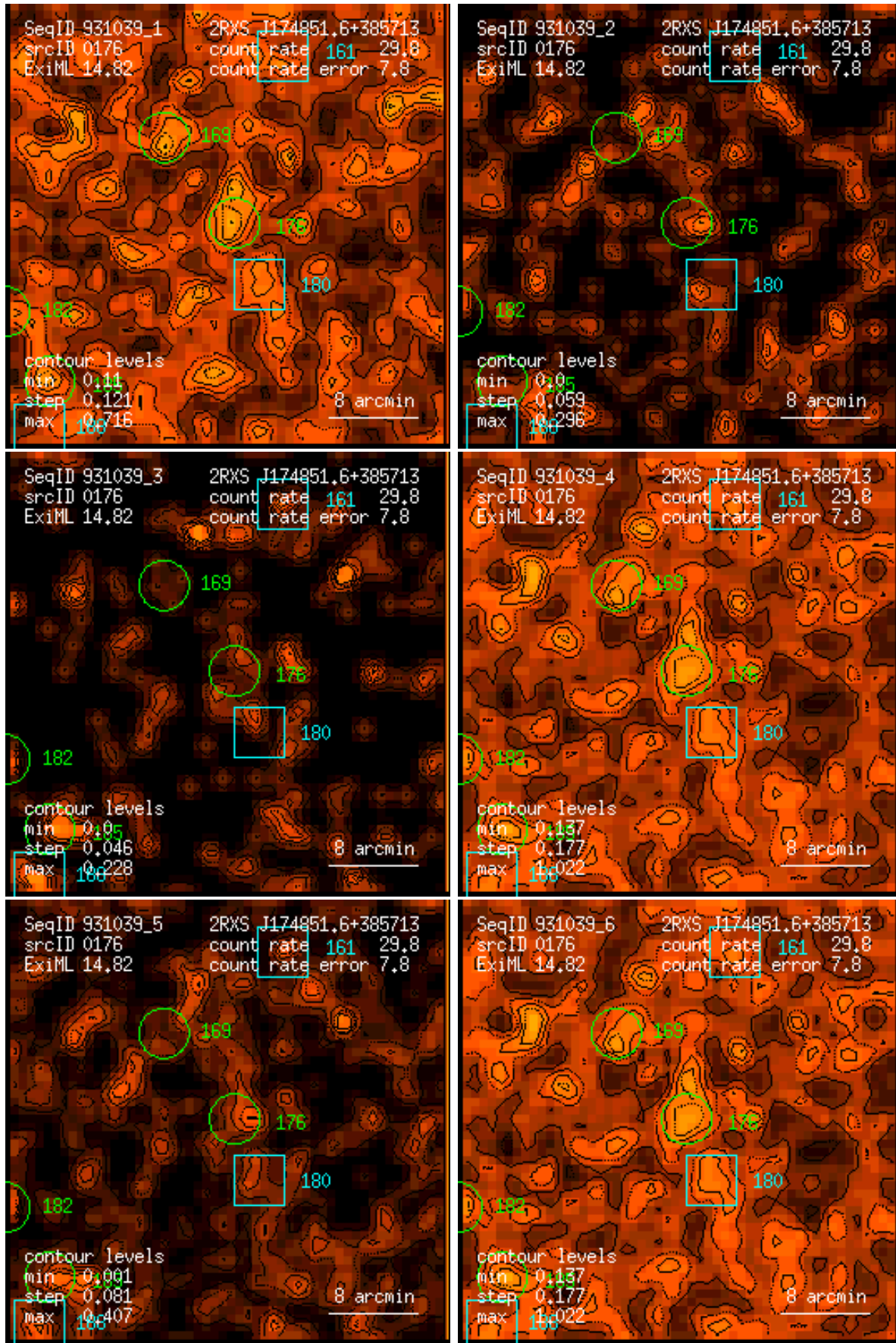
Figure 176: RASS 931039: detection 0176: band rate images, Gaussian filter: (1) PSPC channels 11 – 41, (2) 52 – 90, (3) 91 – 201, (4) 11 – 235, (5) 52 – 201, (6) 11 – 201. Broad band rates in counts/ks. Band rate contour levels in counts/ks/arcmin 2 .
