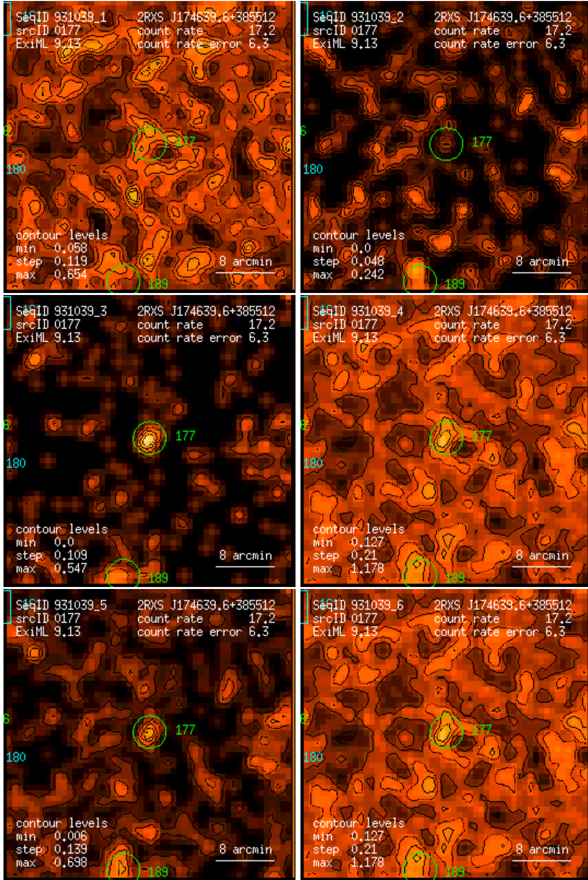
Figure 177: RASS 931039: detection 0177: band rate images, Gaussian filter: (1) PSPC channels 11 – 41, (2) 52 – 90, (3) 91 – 201, (4) 11 – 235, (5) 52 – 201, (6) 11 – 201. Broad band rates in counts/ks. Band rate contour levels in counts/ks/arcmin 2 .
