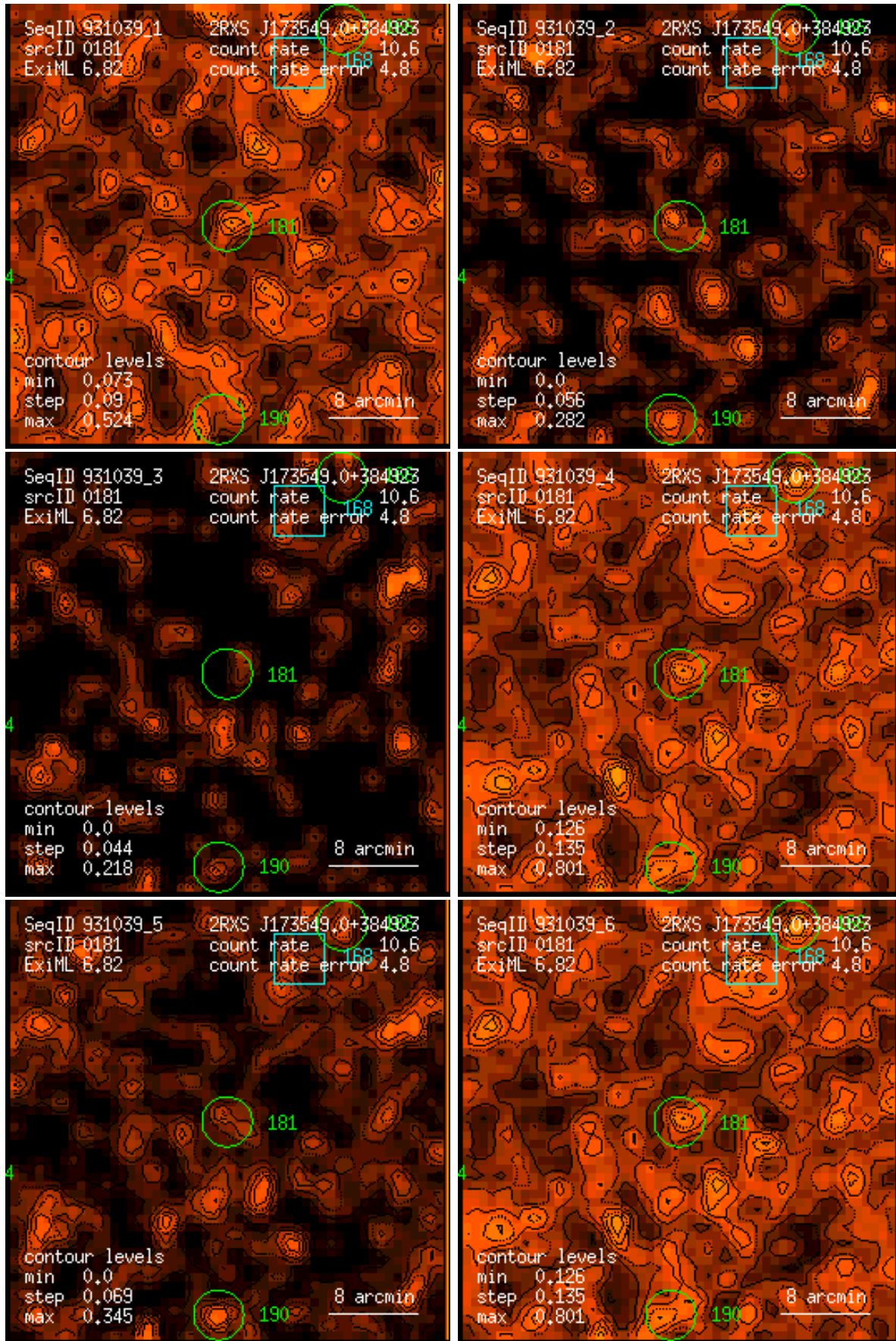
Figure 181: RASS 931039: detection 0181: band rate images, Gaussian filter: (1) PSPC channels 11 – 41, (2) 52 – 90, (3) 91 – 201, (4) 11 – 235, (5) 52 – 201, (6) 11 – 201. Broad band rates in counts/ks. Band rate contour levels in counts/ks/arcmin 2 .
