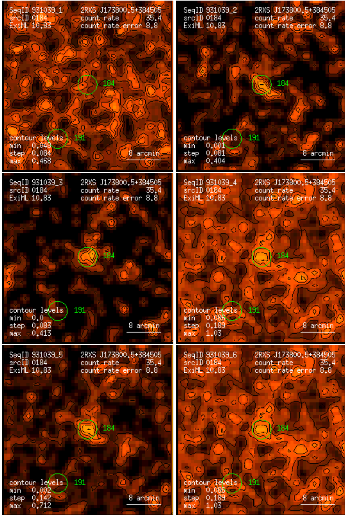
Figure 184: RASS 931039: detection 0184: band rate images, Gaussian filter: (1) PSPC channels 11 – 41, (2) 52 – 90, (3) 91 – 201, (4) 11 – 235, (5) 52 – 201, (6) 11 – 201. Broad band rates in counts/ks. Band rate contour levels in counts/ks/arcmin 2 .
