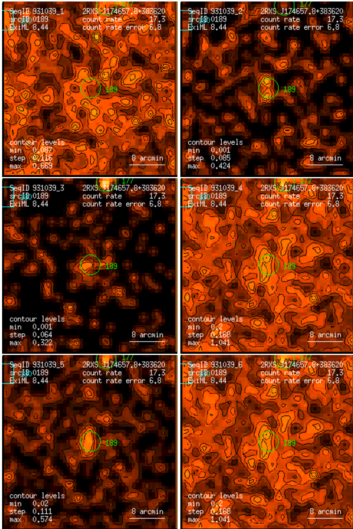
Figure 189: RASS 931039: detection 0189: band rate images, Gaussian filter: (1) PSPC channels 11 – 41, (2) 52 – 90, (3) 91 – 201, (4) 11 – 235, (5) 52 – 201, (6) 11 – 201. Broad band rates in counts/ks. Band rate contour levels in counts/ks/arcmin 2 .
