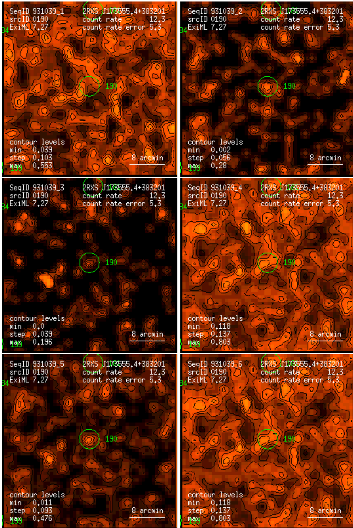
Figure 190: RASS 931039: detection 0190: band rate images, Gaussian filter: (1) PSPC channels 11 – 41, (2) 52 – 90, (3) 91 – 201, (4) 11 – 235, (5) 52 – 201, (6) 11 – 201. Broad band rates in counts/ks. Band rate contour levels in counts/ks/arcmin 2 .
