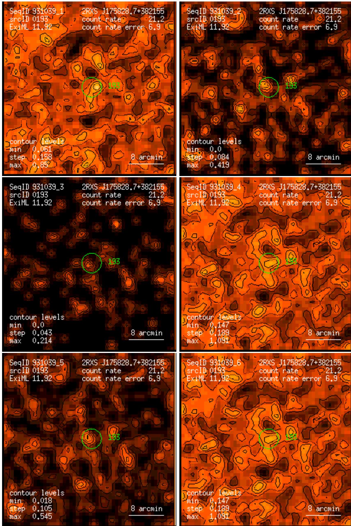
Figure 193: RASS 931039: detection 0193: band rate images, Gaussian filter: (1) PSPC channels 11 – 41, (2) 52 – 90, (3) 91 – 201, (4) 11 – 235, (5) 52 – 201, (6) 11 – 201. Broad band rates in counts/ks. Band rate contour levels in counts/ks/arcmin 2 .
