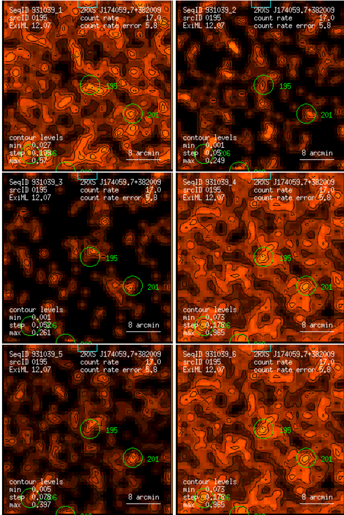
Figure 195: RASS 931039: detection 0195: band rate images, Gaussian filter: (1) PSPC channels 11 – 41, (2) 52 – 90, (3) 91 – 201, (4) 11 – 235, (5) 52 – 201, (6) 11 – 201. Broad band rates in counts/ks. Band rate contour levels in counts/ks/arcmin 2 .
