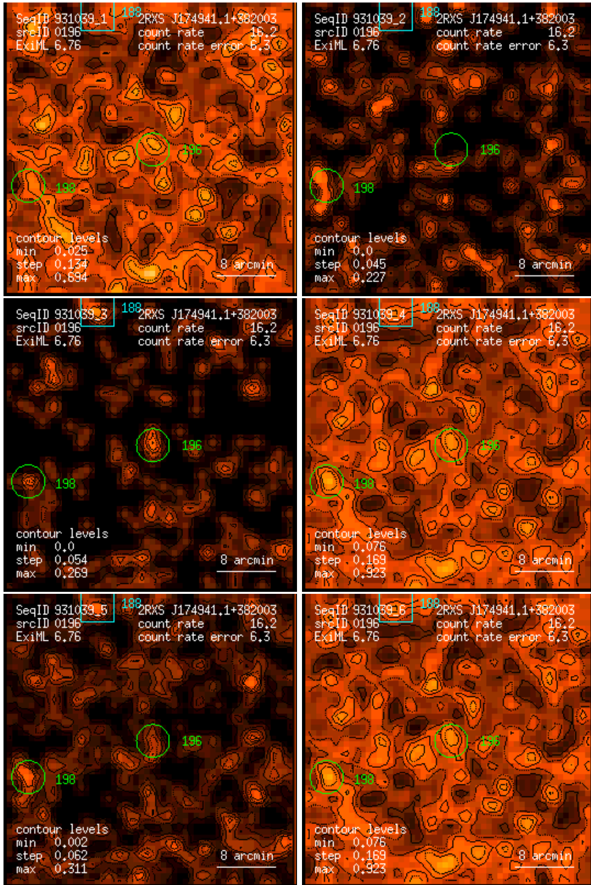
Figure 196: RASS 931039: detection 0196: band rate images, Gaussian filter: (1) PSPC channels 11 – 41, (2) 52 – 90, (3) 91 – 201, (4) 11 – 235, (5) 52 – 201, (6) 11 – 201. Broad band rates in counts/ks. Band rate contour levels in counts/ks/arcmin 2 .
