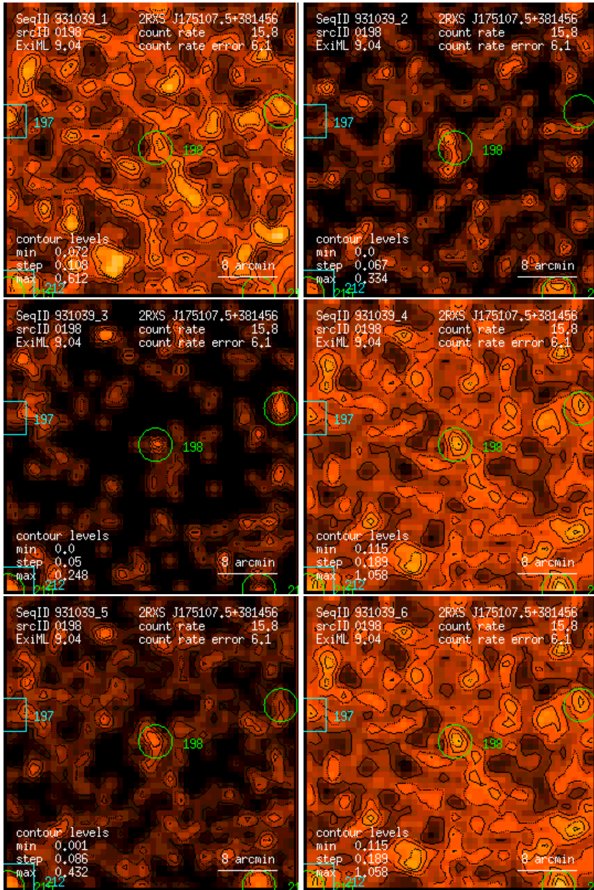
Figure 198: RASS 931039: detection 0198: band rate images, Gaussian filter: (1) PSPC channels 11 – 41, (2) 52 – 90, (3) 91 – 201, (4) 11 – 235, (5) 52 – 201, (6) 11 – 201. Broad band rates in counts/ks. Band rate contour levels in counts/ks/arcmin 2 .
