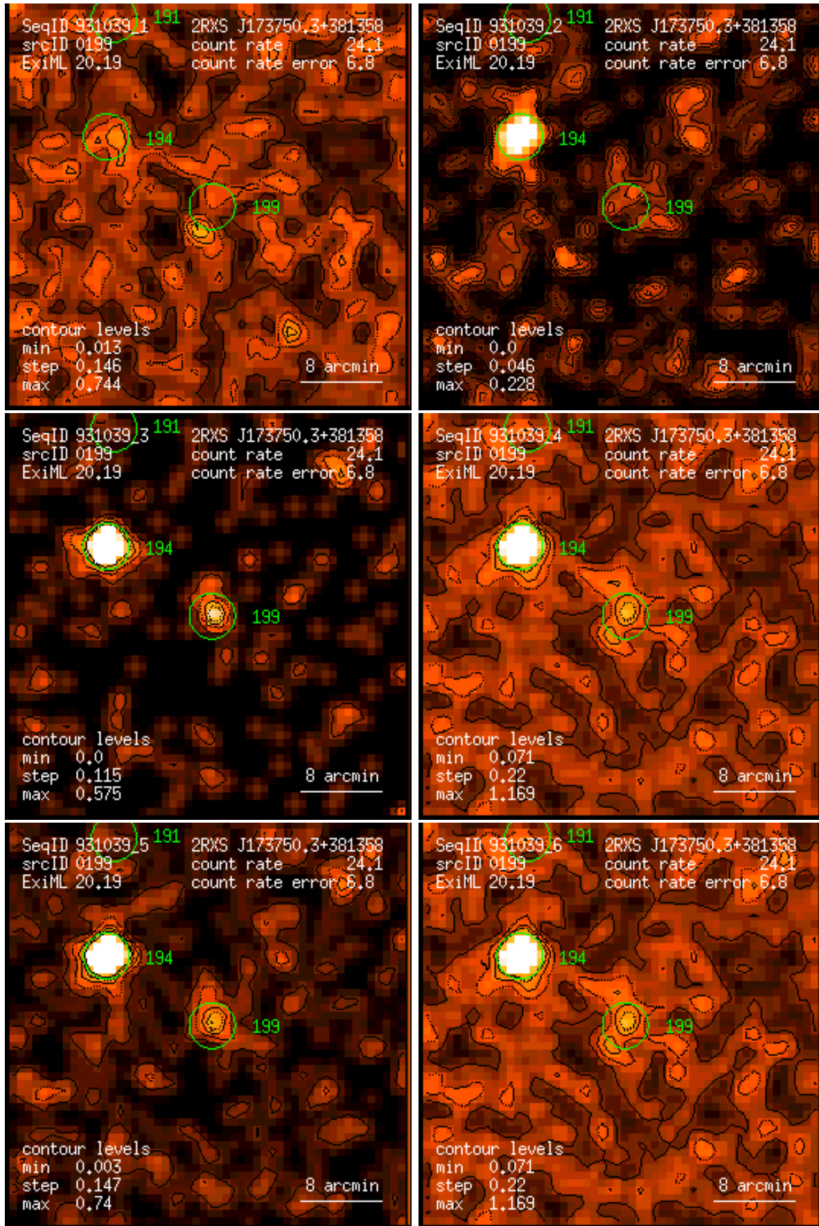
Figure 199: RASS 931039: detection 0199: band rate images, Gaussian filter: (1) PSPC channels 11 – 41, (2) 52 – 90, (3) 91 – 201, (4) 11 – 235, (5) 52 – 201, (6) 11 – 201. Broad band rates in counts/ks. Band rate contour levels in counts/ks/arcmin 2 .
