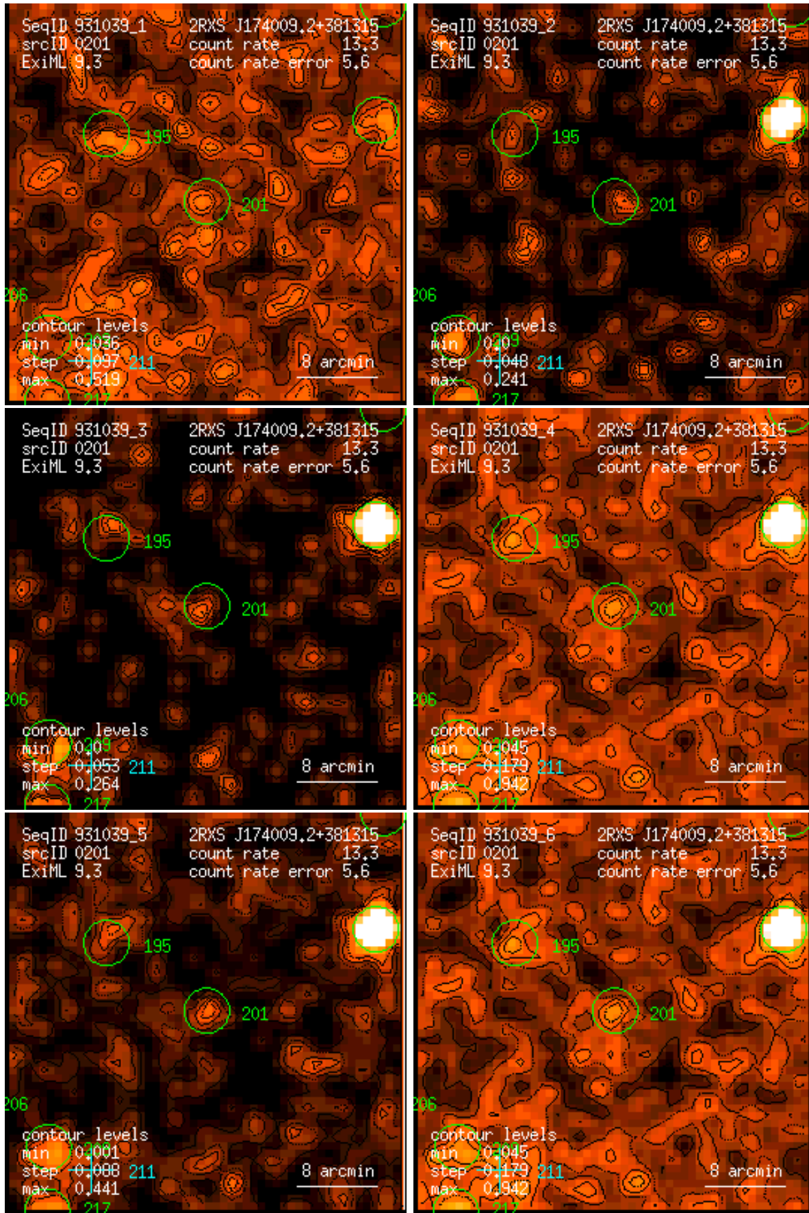
Figure 201: RASS 931039: detection 0201: band rate images, Gaussian filter: (1) PSPC channels 11 – 41, (2) 52 – 90, (3) 91 – 201, (4) 11 – 235, (5) 52 – 201, (6) 11 – 201. Broad band rates in counts/ks. Band rate contour levels in counts/ks/arcmin 2 .
