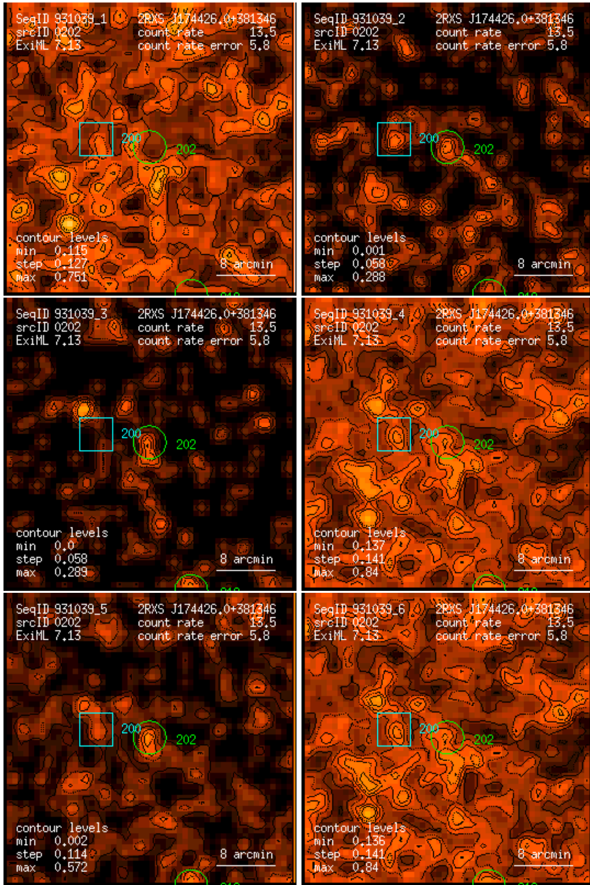
Figure 202: RASS 931039: detection 0202: band rate images, Gaussian filter: (1) PSPC channels 11 – 41, (2) 52 – 90, (3) 91 – 201, (4) 11 – 235, (5) 52 – 201, (6) 11 – 201. Broad band rates in counts/ks. Band rate contour levels in counts/ks/arcmin 2 .
