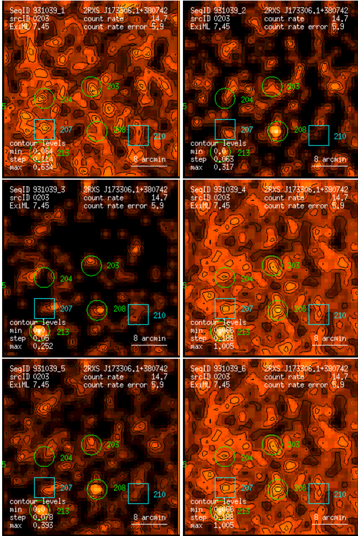
Figure 203: RASS 931039: detection 0203: band rate images, Gaussian filter: (1) PSPC channels 11 – 41, (2) 52 – 90, (3) 91 – 201, (4) 11 – 235, (5) 52 – 201, (6) 11 – 201. Broad band rates in counts/ks. Band rate contour levels in counts/ks/arcmin 2 .
