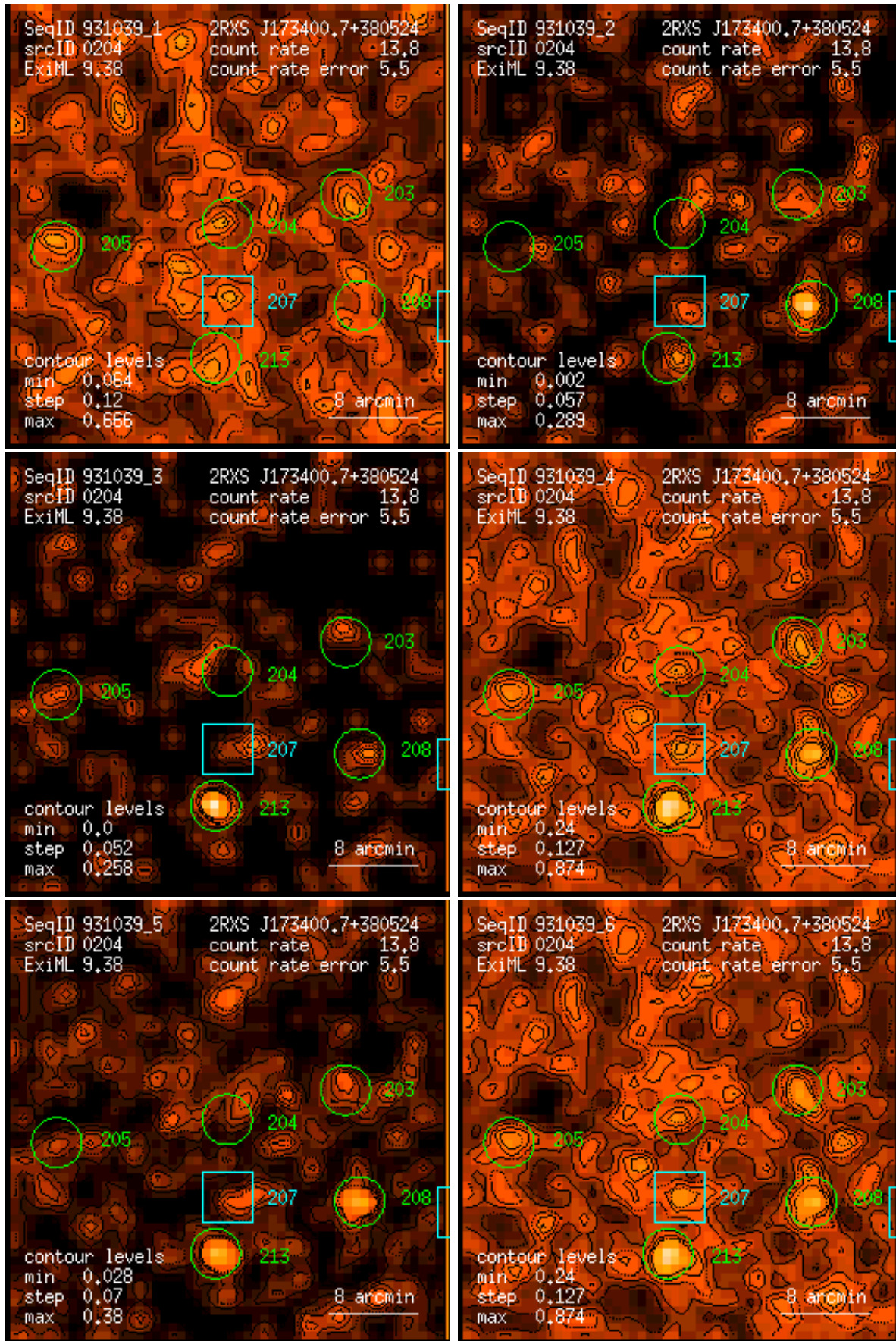
Figure 204: RASS 931039: detection 0204: band rate images, Gaussian filter: (1) PSPC channels 11 – 41, (2) 52 – 90, (3) 91 – 201, (4) 11 – 235, (5) 52 – 201, (6) 11 – 201. Broad band rates in counts/ks. Band rate contour levels in counts/ks/arcmin 2 .
