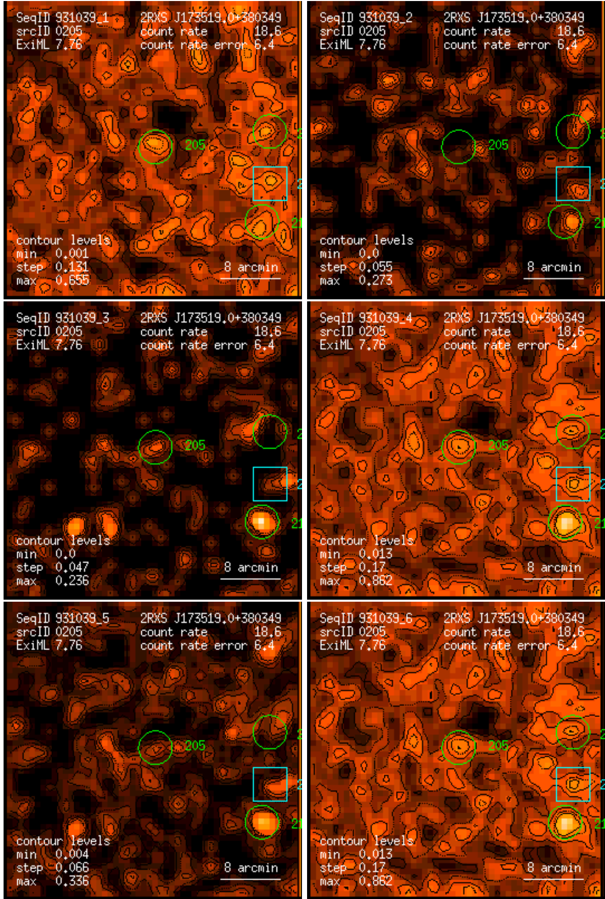
Figure 205: RASS 931039: detection 0205: band rate images, Gaussian filter: (1) PSPC channels 11 – 41, (2) 52 – 90, (3) 91 – 201, (4) 11 – 235, (5) 52 – 201, (6) 11 – 201. Broad band rates in counts/ks. Band rate contour levels in counts/ks/arcmin 2 .
