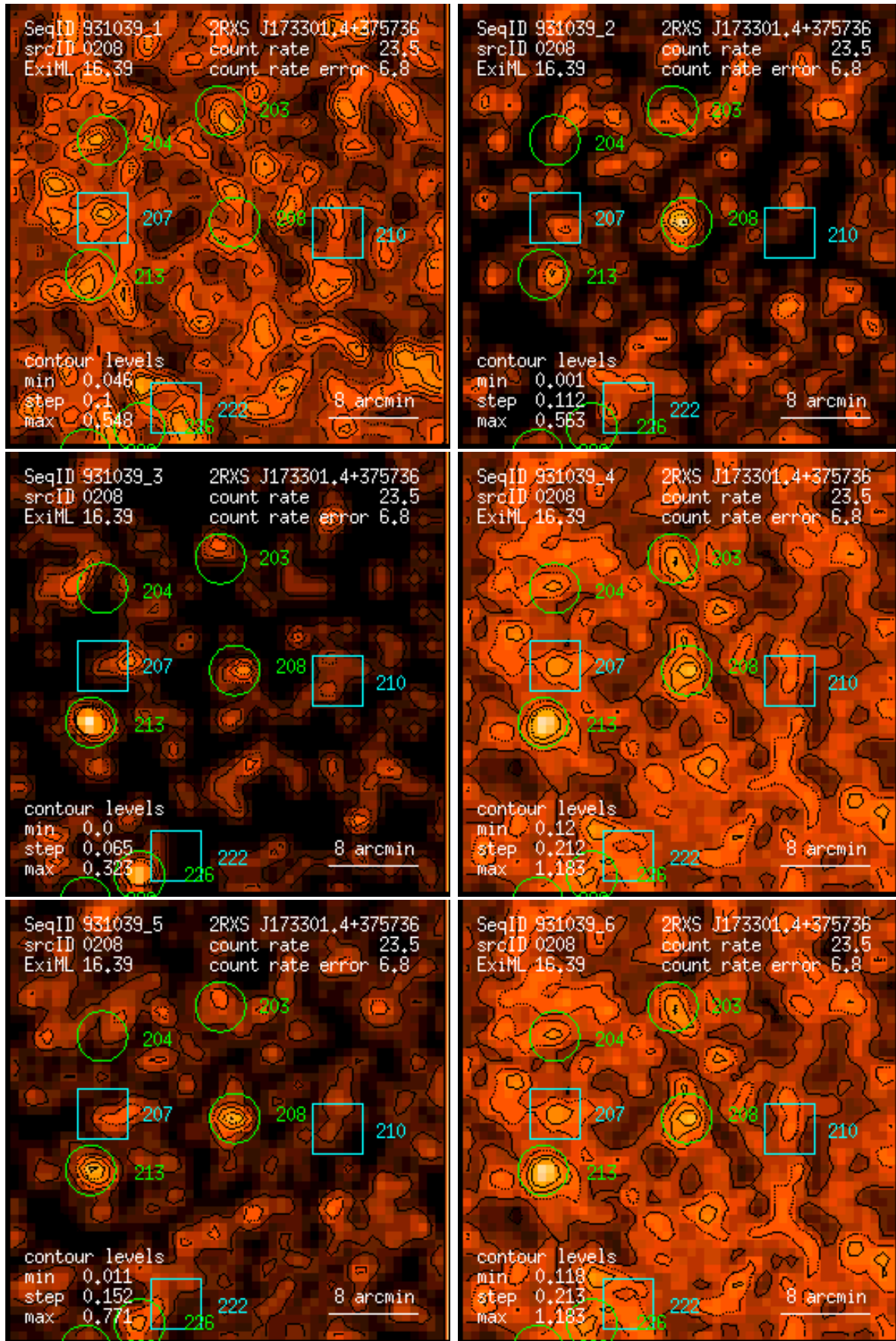
Figure 208: RASS 931039: detection 0208: band rate images, Gaussian filter: (1) PSPC channels 11 – 41, (2) 52 – 90, (3) 91 – 201, (4) 11 – 235, (5) 52 – 201, (6) 11 – 201. Broad band rates in counts/ks. Band rate contour levels in counts/ks/arcmin 2 .
