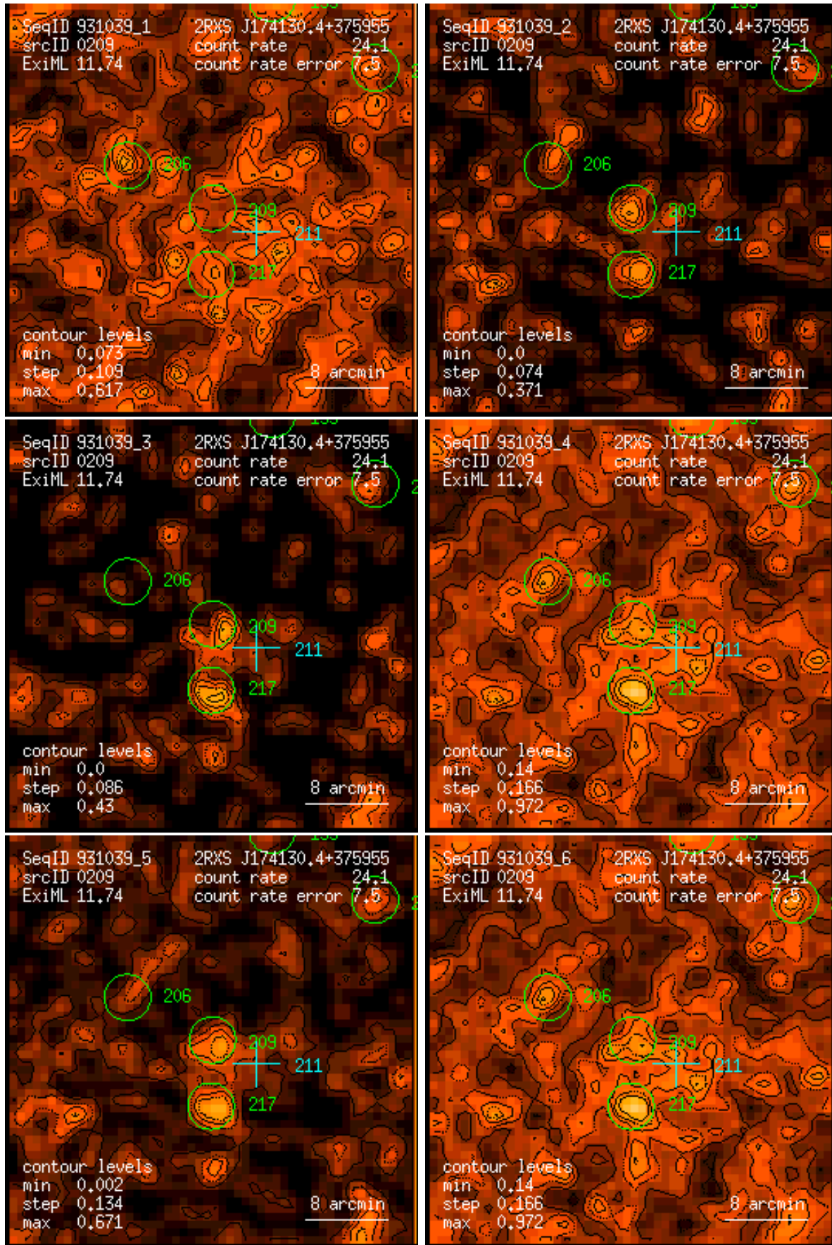
Figure 209: RASS 931039: detection 0209: band rate images, Gaussian filter: (1) PSPC channels 11 – 41, (2) 52 – 90, (3) 91 – 201, (4) 11 – 235, (5) 52 – 201, (6) 11 – 201. Broad band rates in counts/ks. Band rate contour levels in counts/ks/arcmin 2 .
