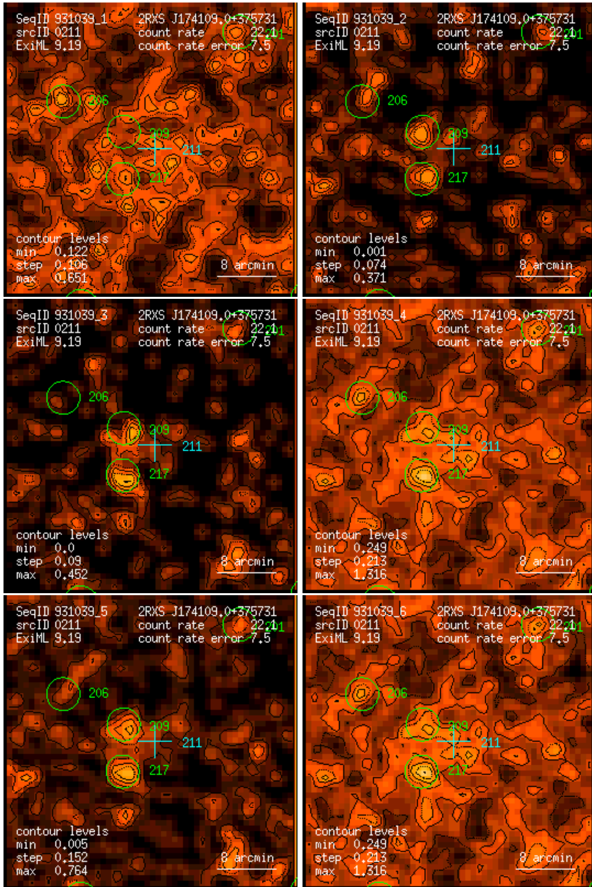
Figure 211: RASS 931039: detection 0211: band rate images, Gaussian filter: (1) PSPC channels 11 – 41, (2) 52 – 90, (3) 91 – 201, (4) 11 – 235, (5) 52 – 201, (6) 11 – 201. Broad band rates in counts/ks. Band rate contour levels in counts/ks/arcmin 2 .
