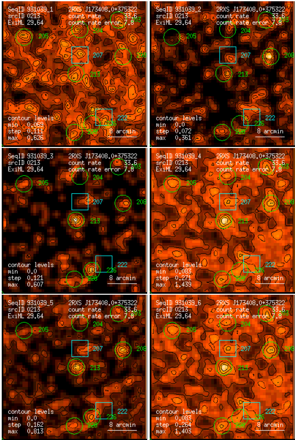
Figure 213: RASS 931039: detection 0213: band rate images, Gaussian filter: (1) PSPC channels 11 – 41, (2) 52 – 90, (3) 91 – 201, (4) 11 – 235, (5) 52 – 201, (6) 11 – 201. Broad band rates in counts/ks. Band rate contour levels in counts/ks/arcmin 2 .
