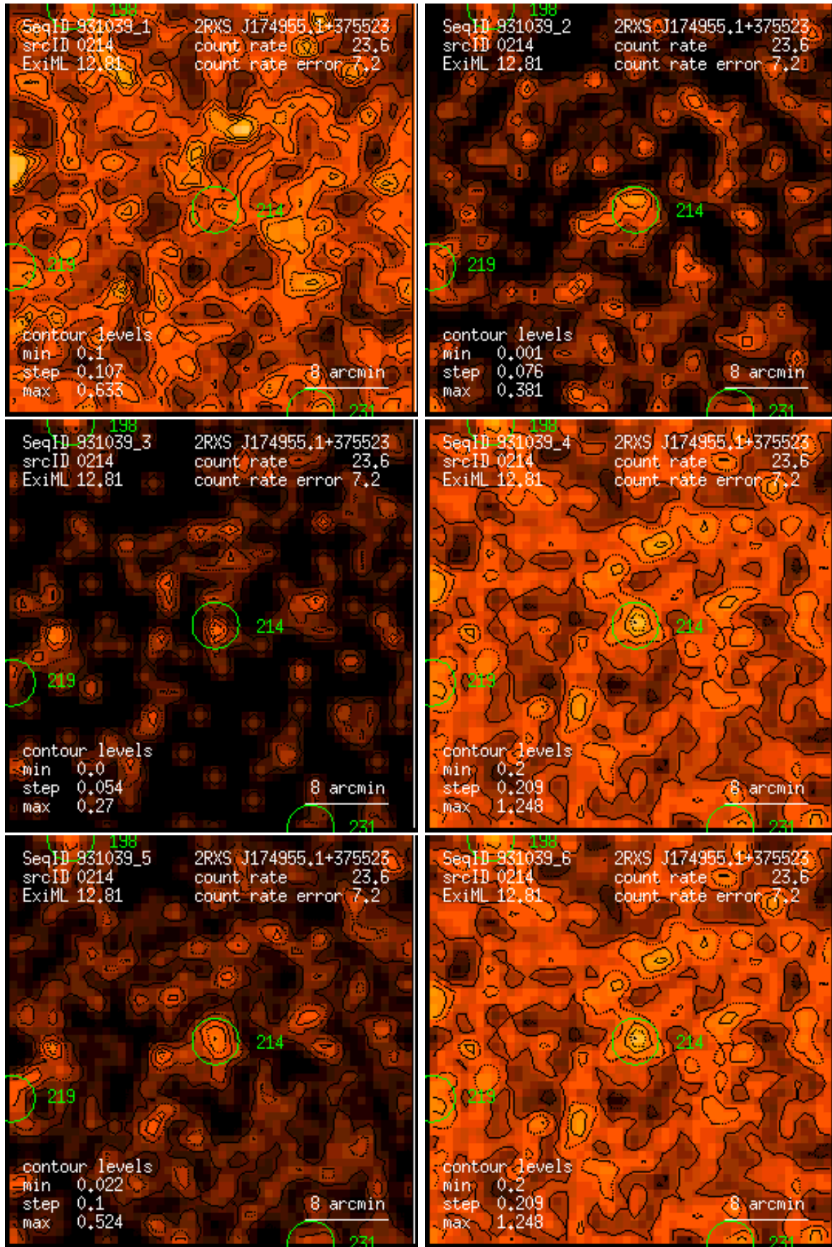
Figure 214: RASS 931039: detection 0214: band rate images, Gaussian filter: (1) PSPC channels 11 – 41, (2) 52 – 90, (3) 91 – 201, (4) 11 – 235, (5) 52 – 201, (6) 11 – 201. Broad band rates in counts/ks. Band rate contour levels in counts/ks/arcmin 2 .
