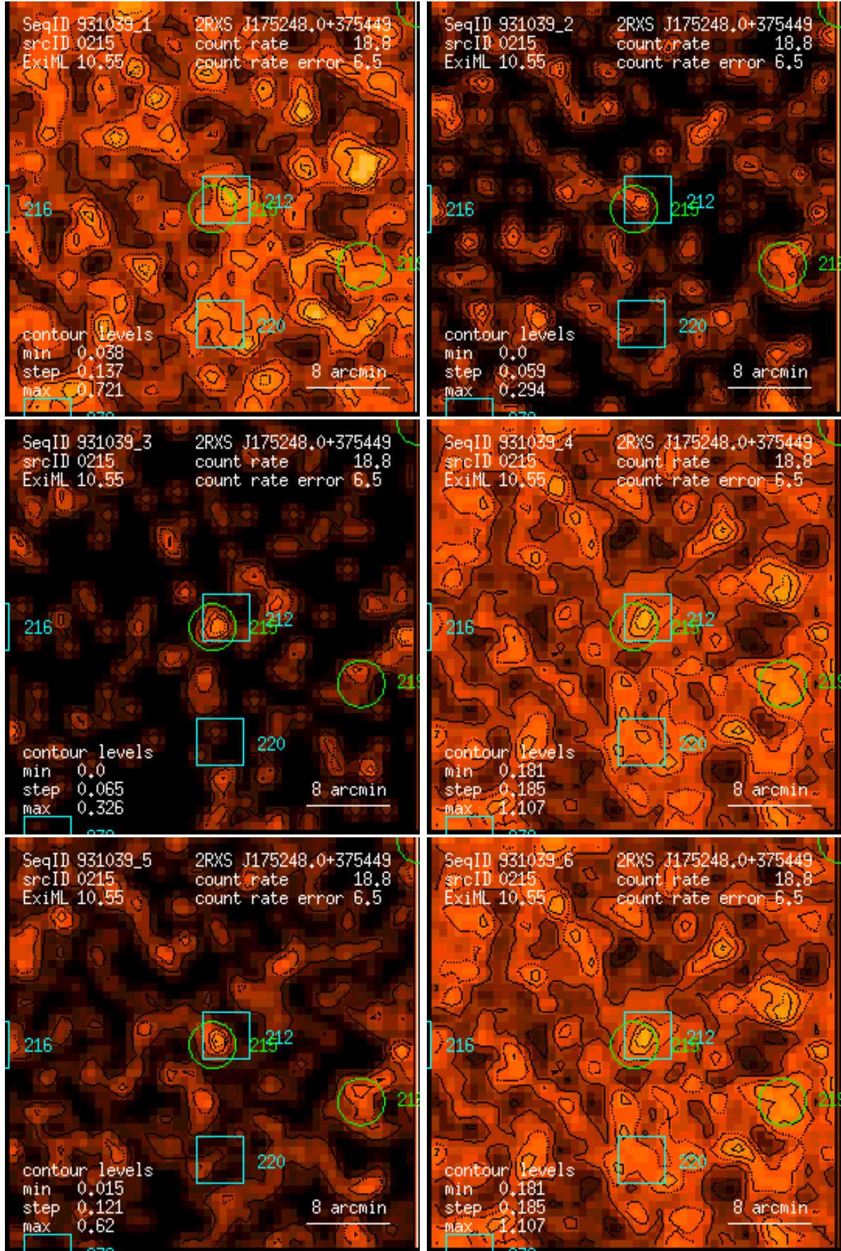
Figure 215: RASS 931039: detection 0215: band rate images, Gaussian filter: (1) PSPC channels 11 – 41, (2) 52 – 90, (3) 91 – 201, (4) 11 – 235, (5) 52 – 201, (6) 11 – 201. Broad band rates in counts/ks. Band rate contour levels in counts/ks/arcmin 2 .
