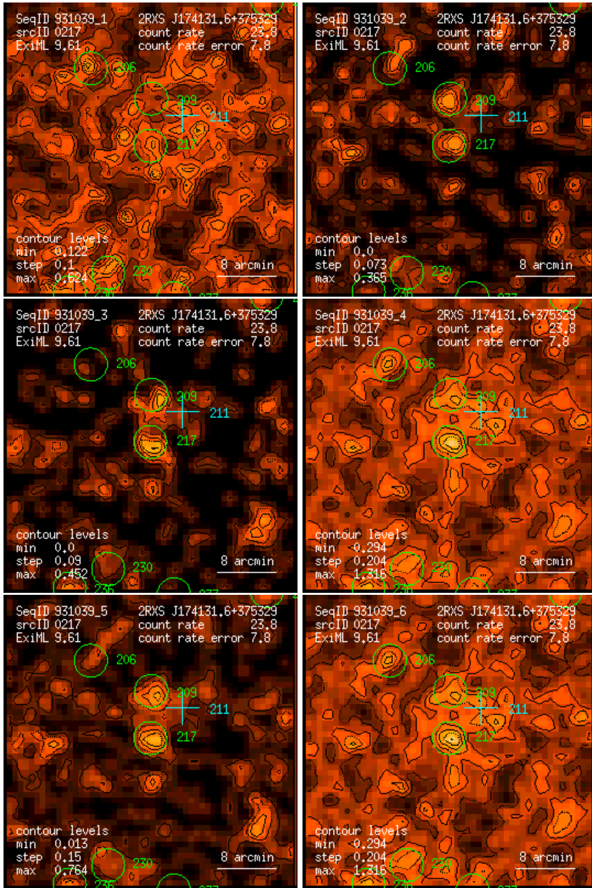
Figure 217: RASS 931039: detection 0217: band rate images, Gaussian filter: (1) PSPC channels 11 – 41, (2) 52 – 90, (3) 91 – 201, (4) 11 – 235, (5) 52 – 201, (6) 11 – 201. Broad band rates in counts/ks. Band rate contour levels in counts/ks/arcmin 2 .
