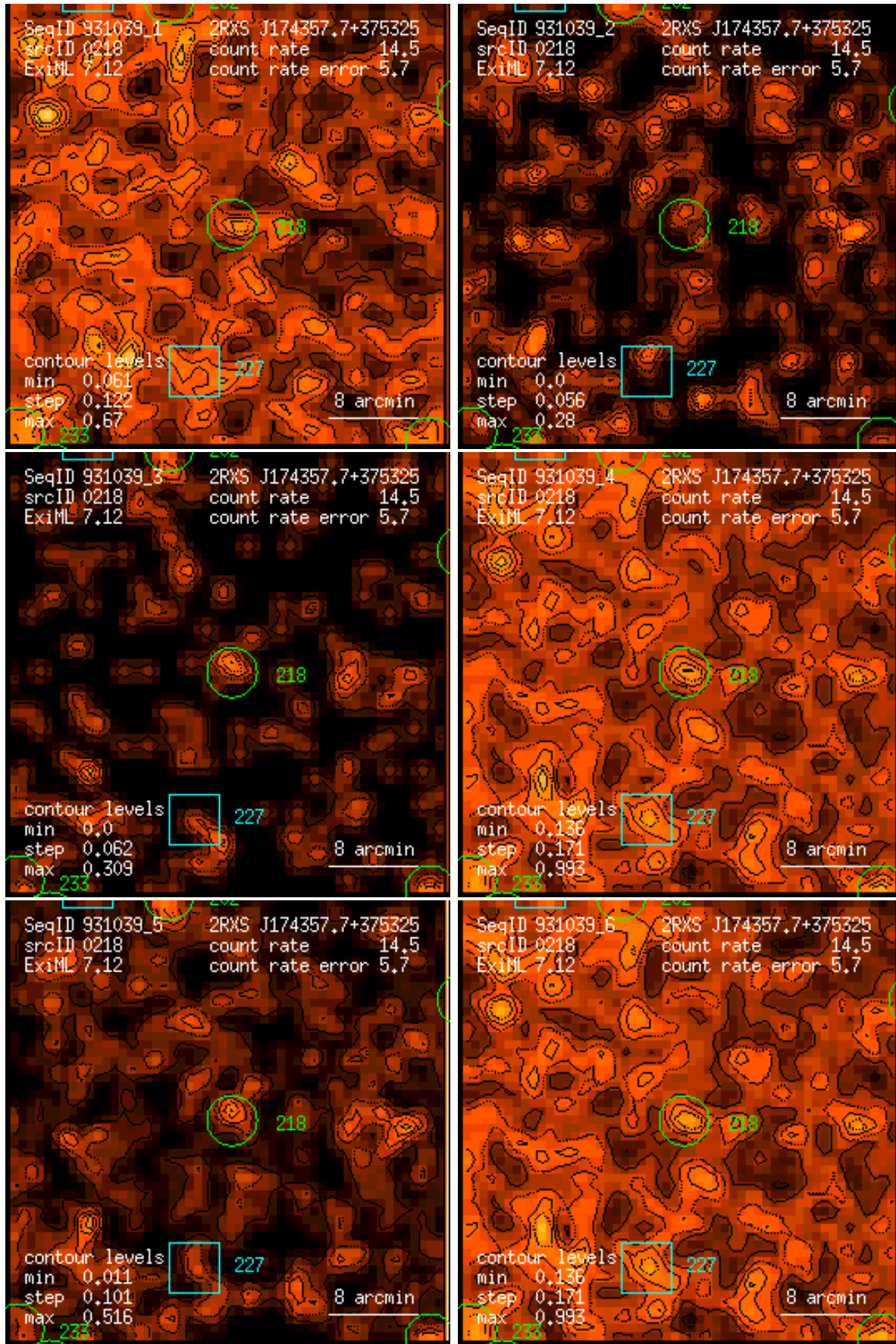
Figure 218: RASS 931039: detection 0218: band rate images, Gaussian filter: (1) PSPC channels 11 – 41, (2) 52 – 90, (3) 91 – 201, (4) 11 – 235, (5) 52 – 201, (6) 11 – 201. Broad band rates in counts/ks. Band rate contour levels in counts/ks/arcmin 2 .
