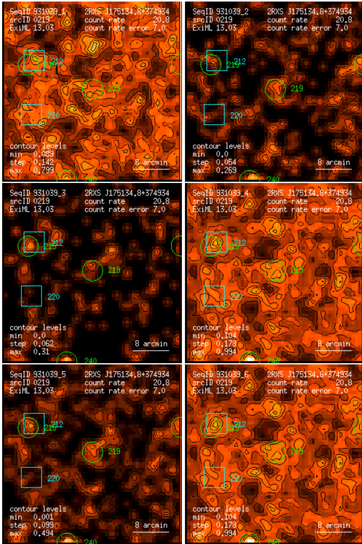
Figure 219: RASS 931039: detection 0219: band rate images, Gaussian filter: (1) PSPC channels 11 – 41, (2) 52 – 90, (3) 91 – 201, (4) 11 – 235, (5) 52 – 201, (6) 11 – 201. Broad band rates in counts/ks. Band rate contour levels in counts/ks/arcmin 2 .
