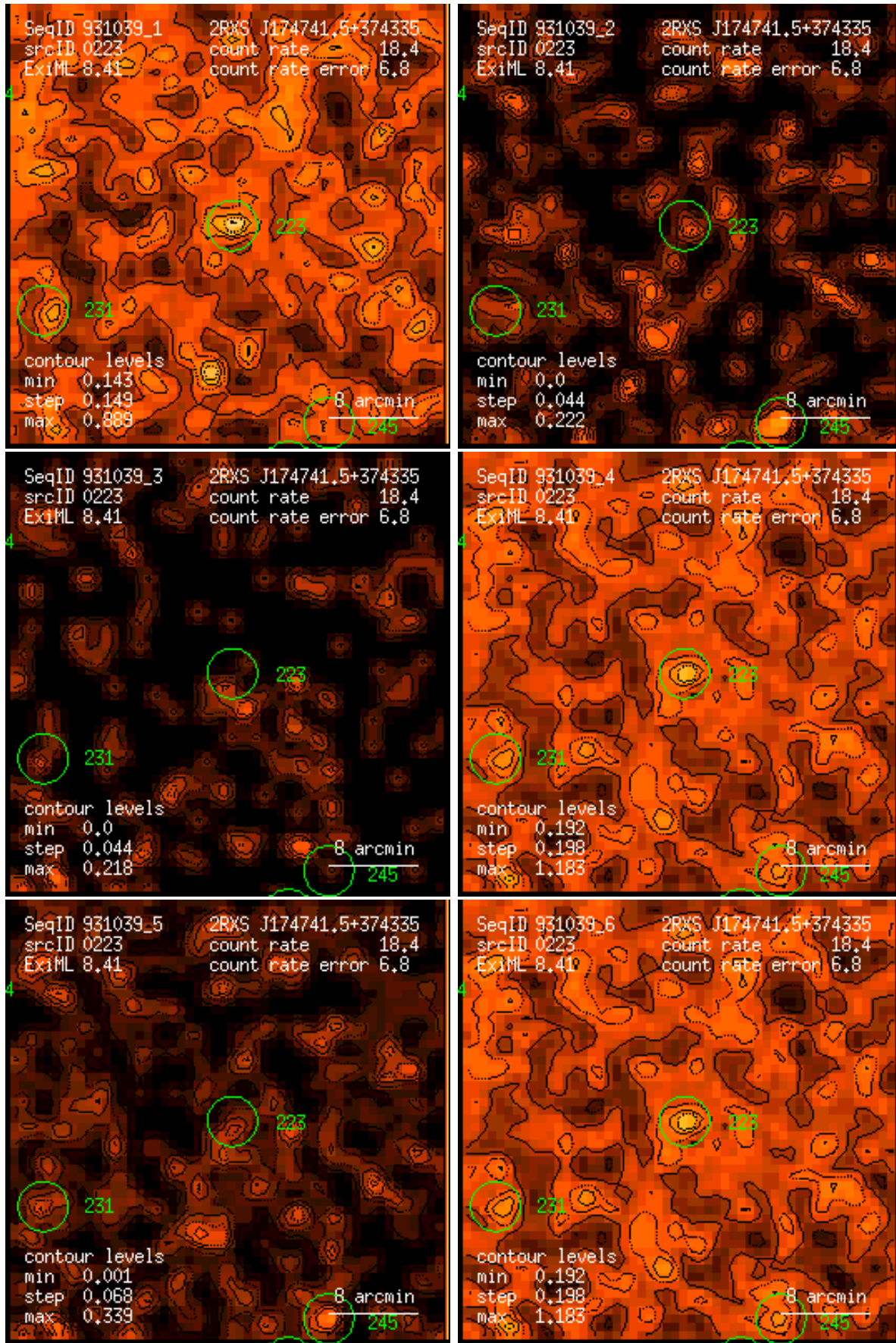
Figure 223: RASS 931039: detection 0223: band rate images, Gaussian filter: (1) PSPC channels 11 – 41, (2) 52 – 90, (3) 91 – 201, (4) 11 – 235, (5) 52 – 201, (6) 11 – 201. Broad band rates in counts/ks. Band rate contour levels in counts/ks/arcmin 2 .
