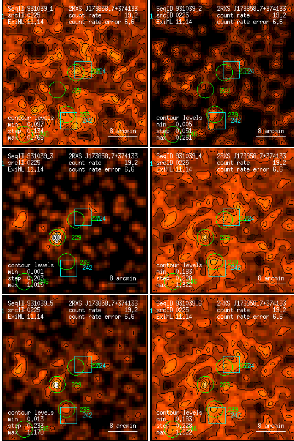
Figure 225: RASS 931039: detection 0225: band rate images, Gaussian filter: (1) PSPC channels 11 – 41, (2) 52 – 90, (3) 91 – 201, (4) 11 – 235, (5) 52 – 201, (6) 11 – 201. Broad band rates in counts/ks. Band rate contour levels in counts/ks/arcmin 2 .
