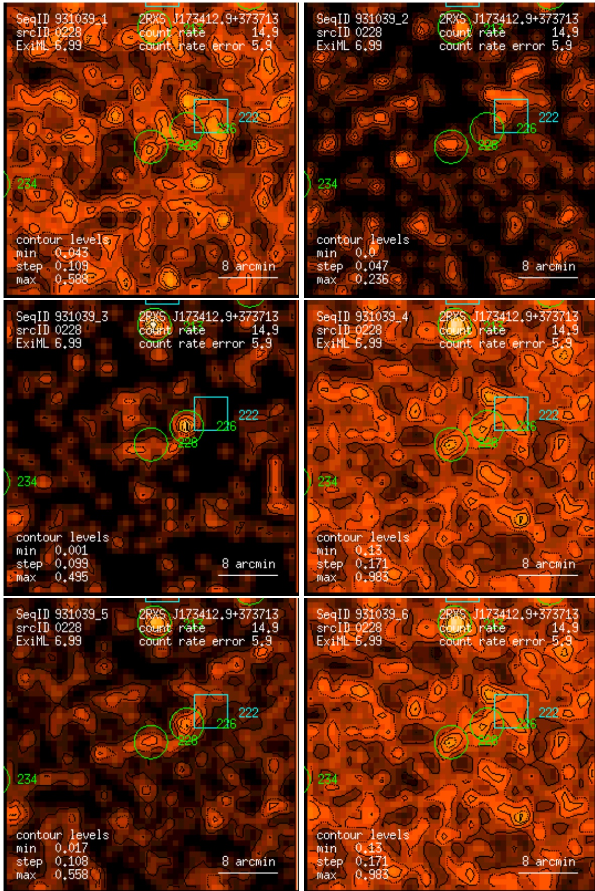
Figure 228: RASS 931039: detection 0228: band rate images, Gaussian filter: (1) PSPC channels 11 – 41, (2) 52 – 90, (3) 91 – 201, (4) 11 – 235, (5) 52 – 201, (6) 11 – 201. Broad band rates in counts/ks. Band rate contour levels in counts/ks/arcmin 2 .
