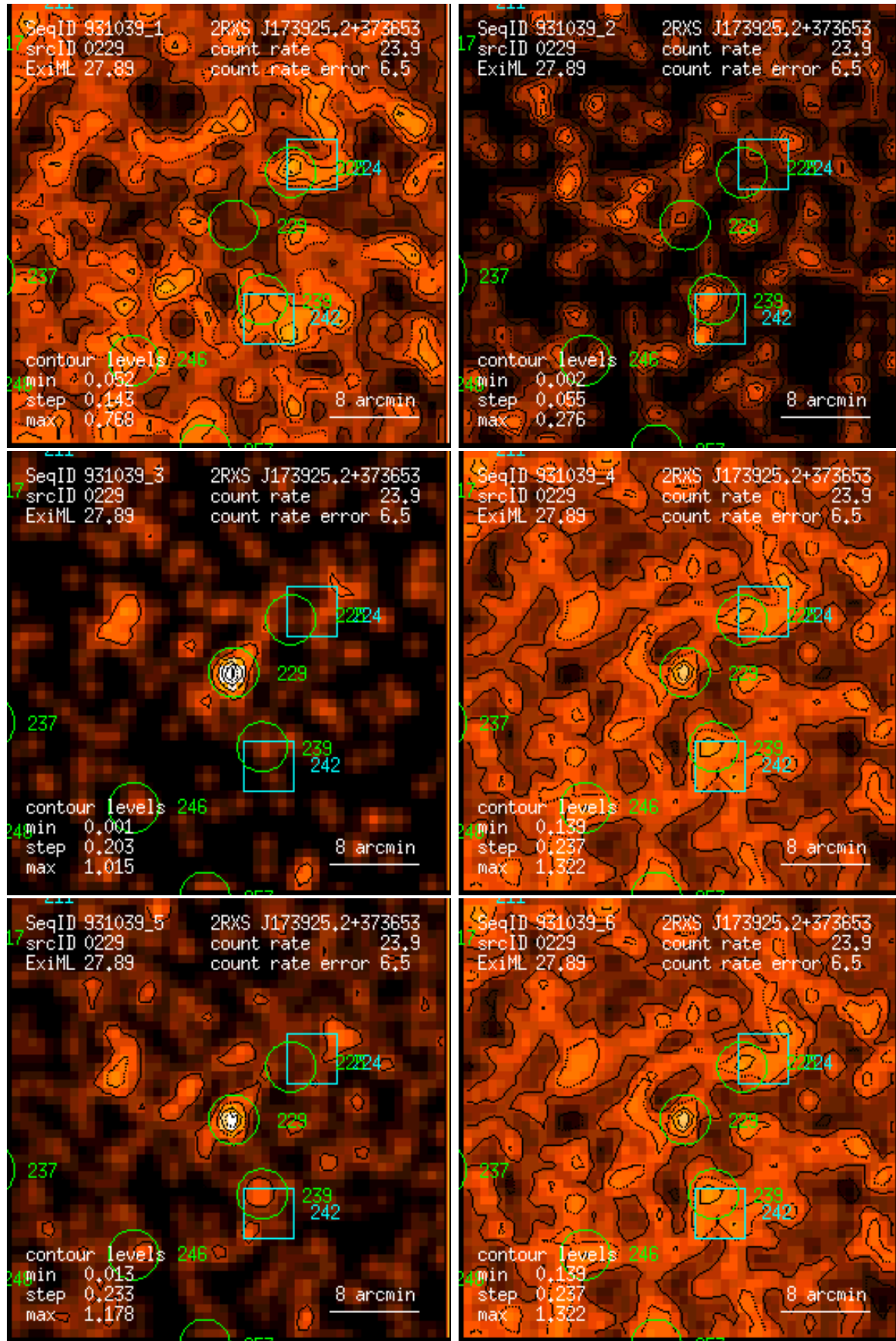
Figure 229: RASS 931039: detection 0229: band rate images, Gaussian filter: (1) PSPC channels 11 – 41, (2) 52 – 90, (3) 91 – 201, (4) 11 – 235, (5) 52 – 201, (6) 11 – 201. Broad band rates in counts/ks. Band rate contour levels in counts/ks/arcmin 2 .
