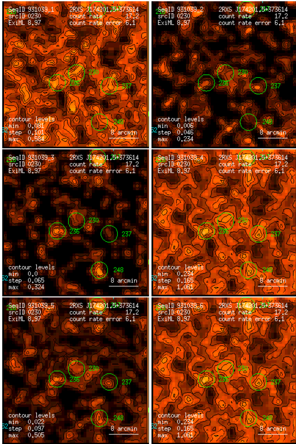
Figure 230: RASS 931039: detection 0230: band rate images, Gaussian filter: (1) PSPC channels 11 – 41, (2) 52 – 90, (3) 91 – 201, (4) 11 – 235, (5) 52 – 201, (6) 11 – 201. Broad band rates in counts/ks. Band rate contour levels in counts/ks/arcmin 2 .
