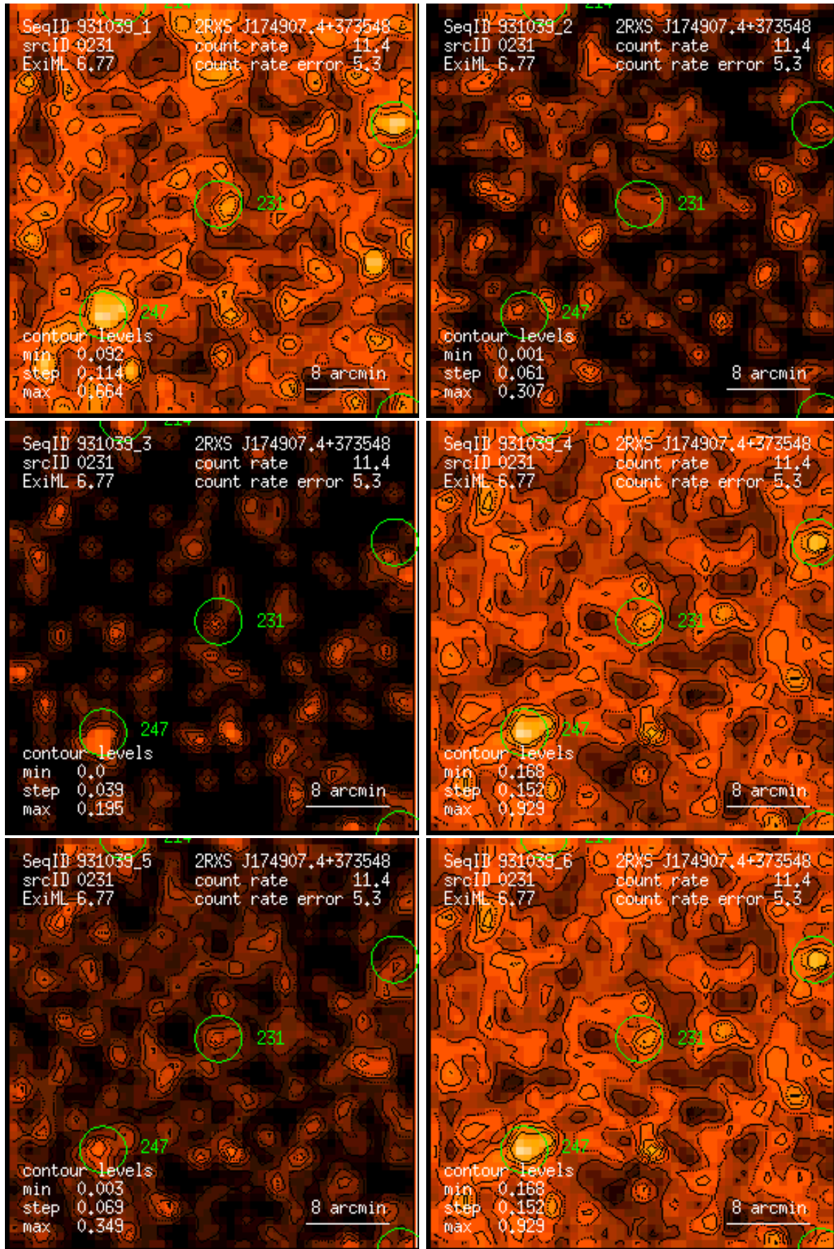
Figure 231: RASS 931039: detection 0231: band rate images, Gaussian filter: (1) PSPC channels 11 – 41, (2) 52 – 90, (3) 91 – 201, (4) 11 – 235, (5) 52 – 201, (6) 11 – 201. Broad band rates in counts/ks. Band rate contour levels in counts/ks/arcmin 2 .
