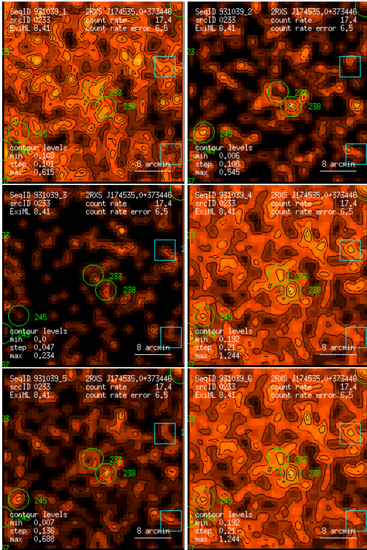
Figure 233: RASS 931039: detection 0233: band rate images, Gaussian filter: (1) PSPC channels 11 – 41, (2) 52 – 90, (3) 91 – 201, (4) 11 – 235, (5) 52 – 201, (6) 11 – 201. Broad band rates in counts/ks. Band rate contour levels in counts/ks/arcmin 2 .
