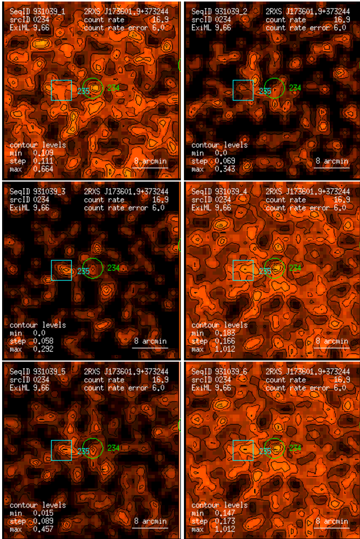
Figure 234: RASS 931039: detection 0234: band rate images, Gaussian filter: (1) PSPC channels 11 – 41, (2) 52 – 90, (3) 91 – 201, (4) 11 – 235, (5) 52 – 201, (6) 11 – 201. Broad band rates in counts/ks. Band rate contour levels in counts/ks/arcmin 2 .
