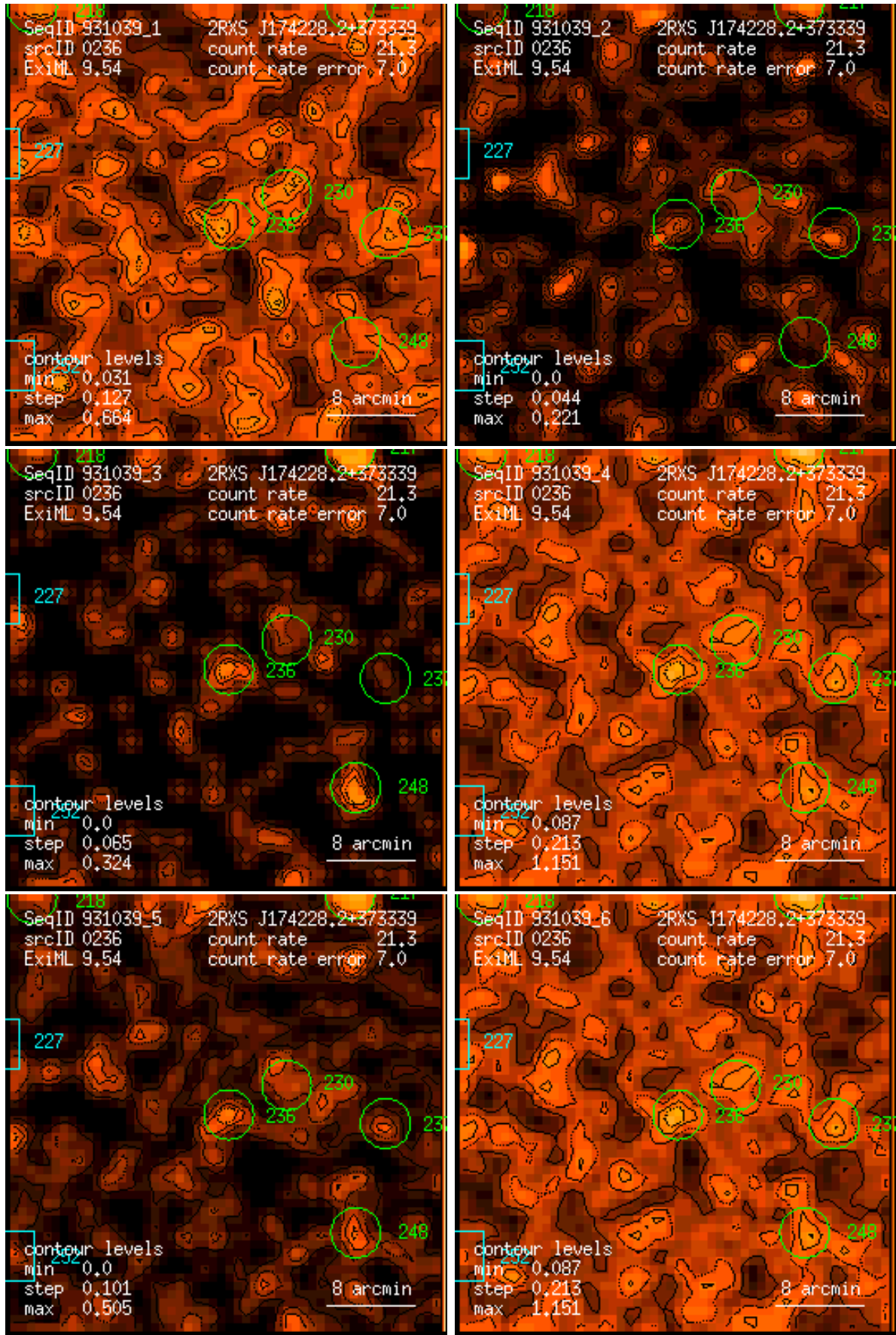
Figure 236: RASS 931039: detection 0236: band rate images, Gaussian filter: (1) PSPC channels 11 – 41, (2) 52 – 90, (3) 91 – 201, (4) 11 – 235, (5) 52 – 201, (6) 11 – 201. Broad band rates in counts/ks. Band rate contour levels in counts/ks/arcmin 2 .
