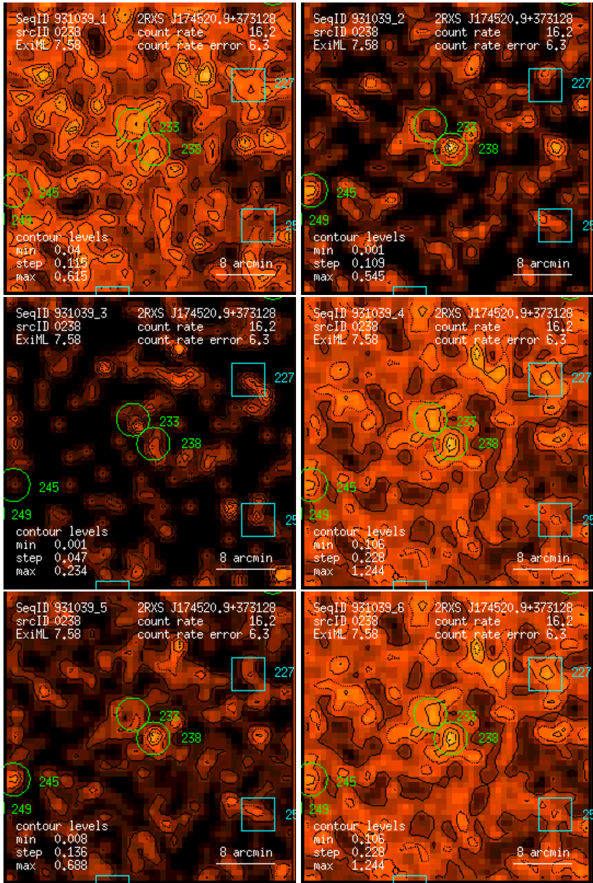
Figure 238: RASS 931039: detection 0238: band rate images, Gaussian filter: (1) PSPC channels 11 – 41, (2) 52 – 90, (3) 91 – 201, (4) 11 – 235, (5) 52 – 201, (6) 11 – 201. Broad band rates in counts/ks. Band rate contour levels in counts/ks/arcmin 2 .
