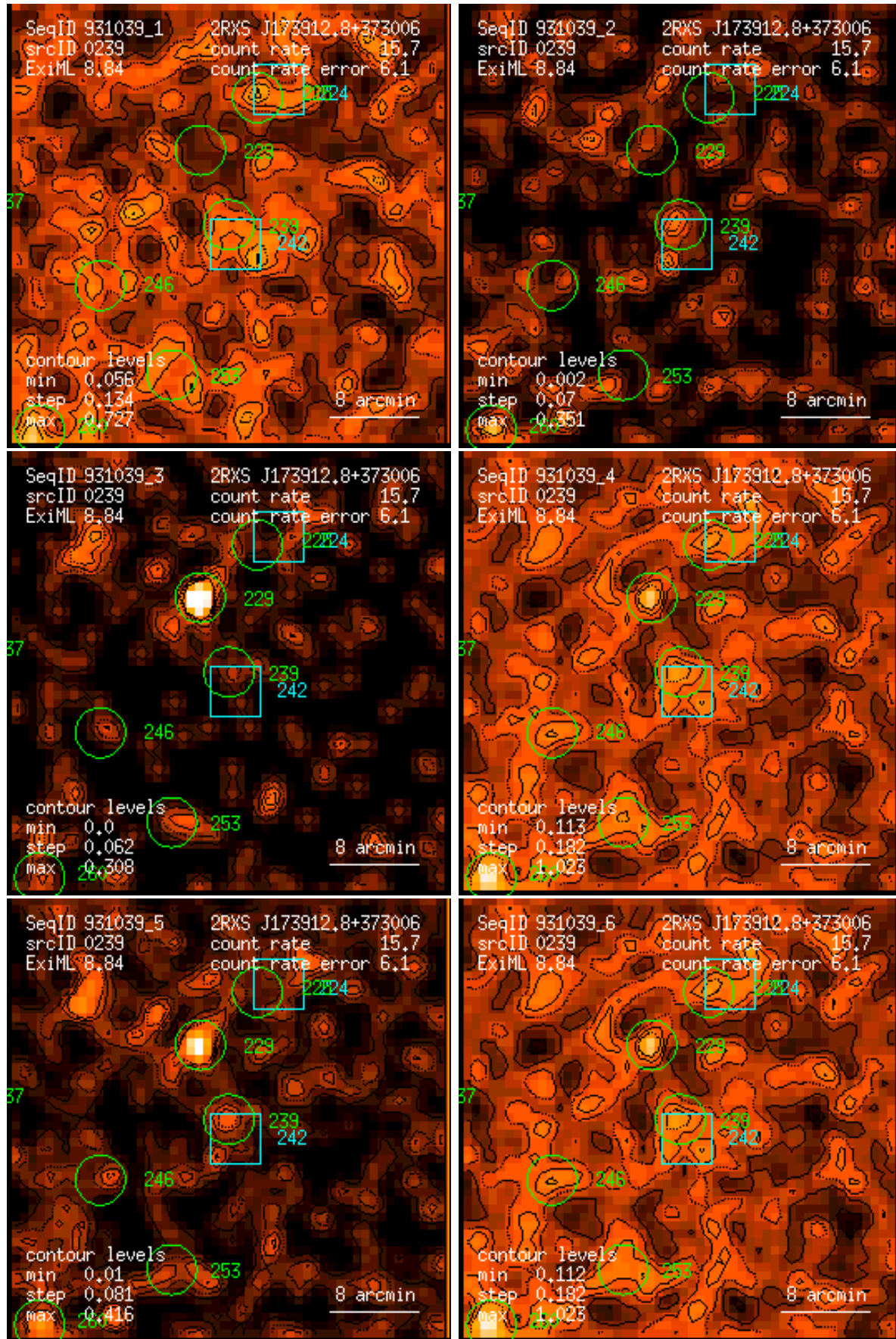
Figure 239: RASS 931039: detection 0239: band rate images, Gaussian filter: (1) PSPC channels 11 – 41, (2) 52 – 90, (3) 91 – 201, (4) 11 – 235, (5) 52 – 201, (6) 11 – 201. Broad band rates in counts/ks. Band rate contour levels in counts/ks/arcmin 2 .
