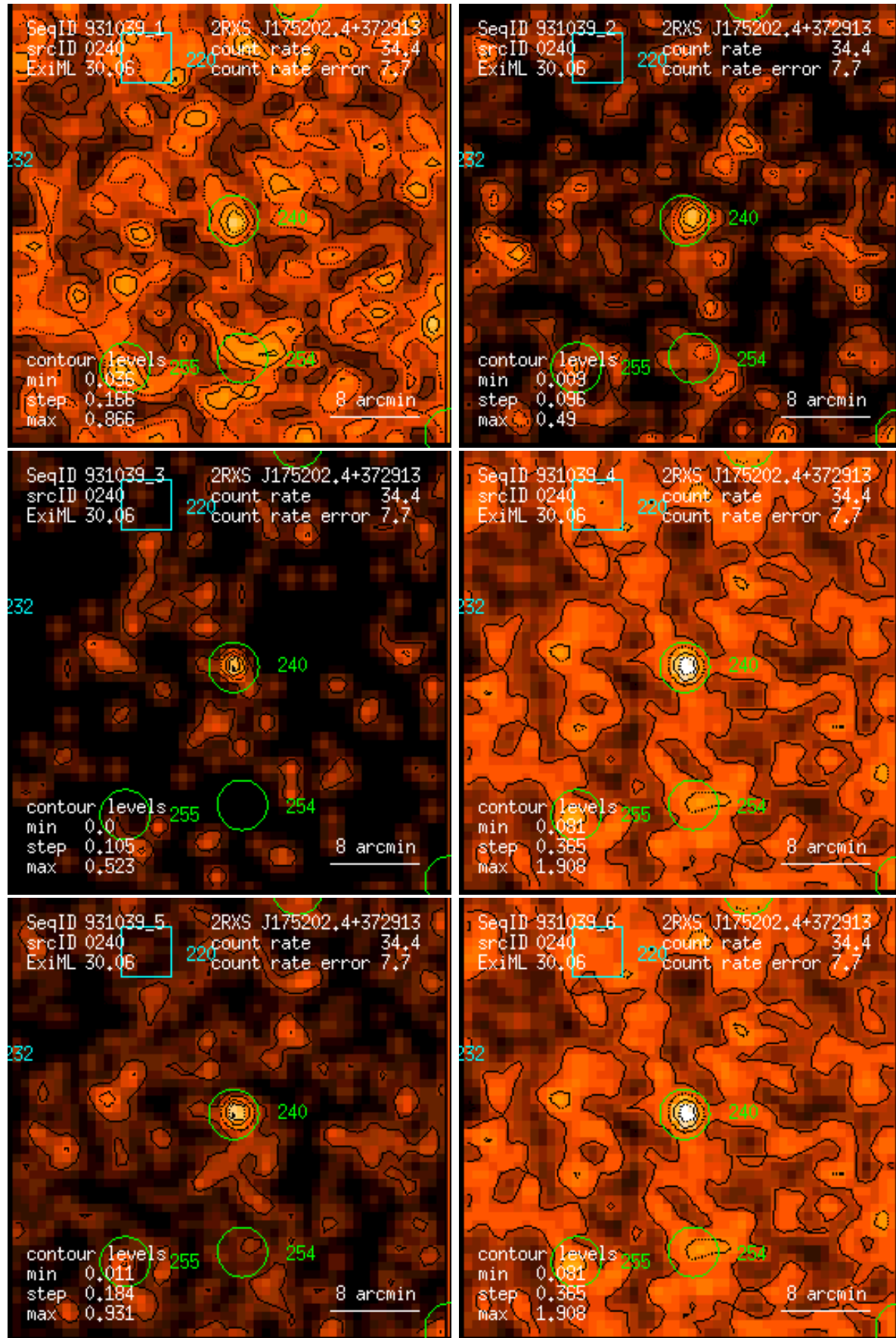
Figure 240: RASS 931039: detection 0240: band rate images, Gaussian filter: (1) PSPC channels 11 – 41, (2) 52 – 90, (3) 91 – 201, (4) 11 – 235, (5) 52 – 201, (6) 11 – 201. Broad band rates in counts/ks. Band rate contour levels in counts/ks/arcmin 2 .
