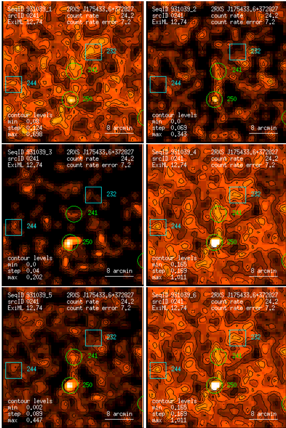
Figure 241: RASS 931039: detection 0241: band rate images, Gaussian filter: (1) PSPC channels 11 – 41, (2) 52 – 90, (3) 91 – 201, (4) 11 – 235, (5) 52 – 201, (6) 11 – 201. Broad band rates in counts/ks. Band rate contour levels in counts/ks/arcmin 2 .
