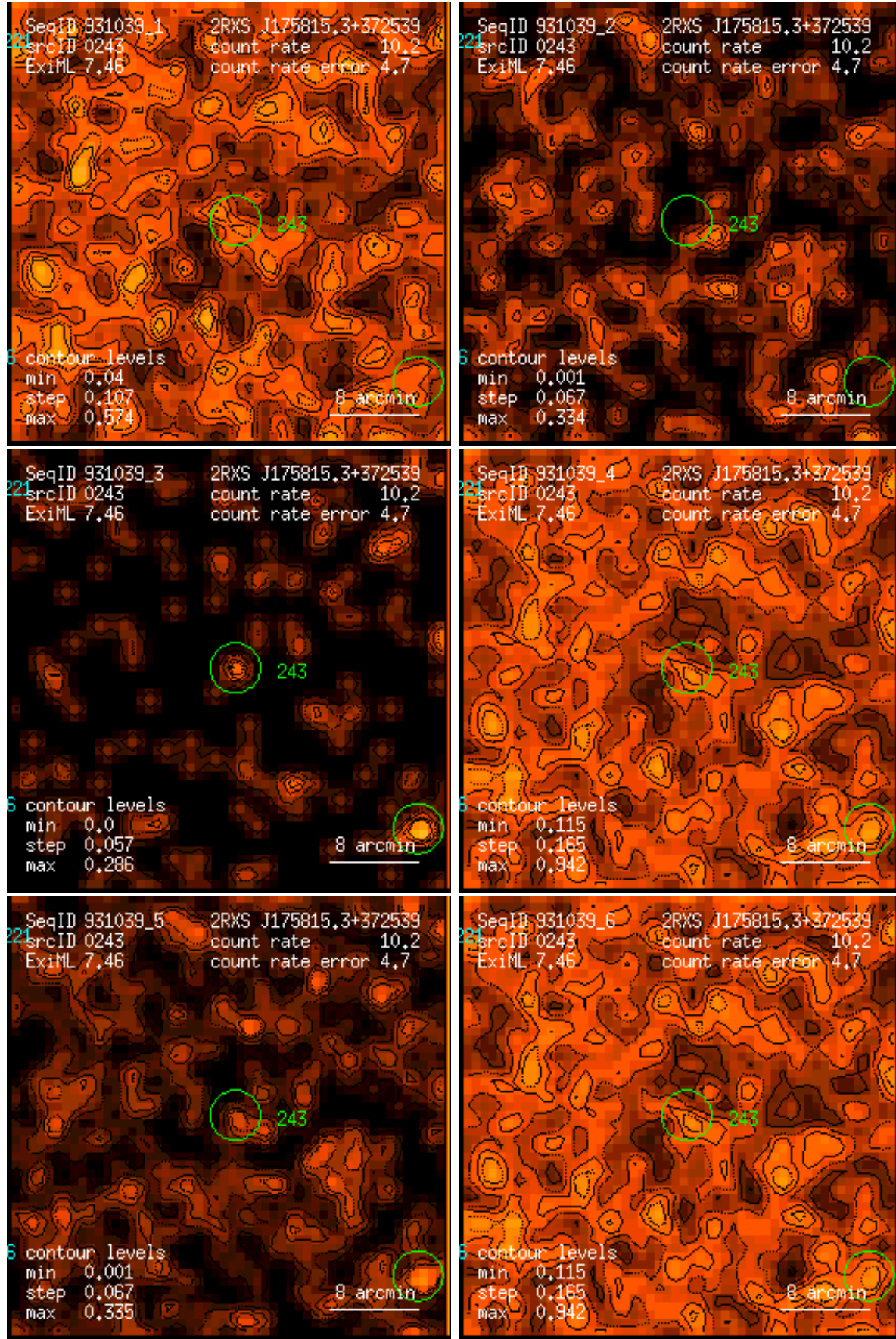
Figure 243: RASS 931039: detection 0243: band rate images, Gaussian filter: (1) PSPC channels 11 – 41, (2) 52 – 90, (3) 91 – 201, (4) 11 – 235, (5) 52 – 201, (6) 11 – 201. Broad band rates in counts/ks. Band rate contour levels in counts/ks/arcmin 2 .
