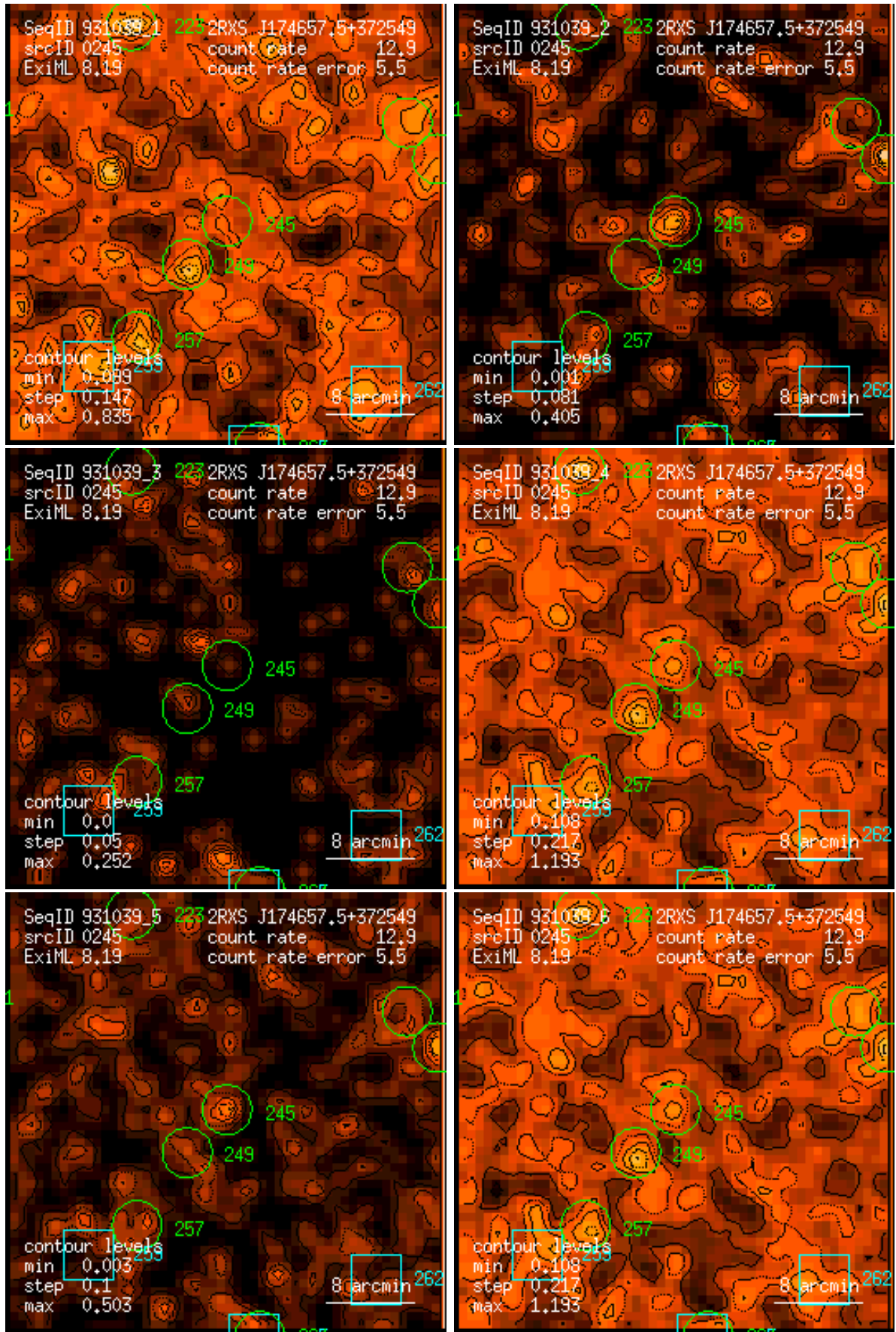
Figure 245: RASS 931039: detection 0245: band rate images, Gaussian filter: (1) PSPC channels 11 – 41, (2) 52 – 90, (3) 91 – 201, (4) 11 – 235, (5) 52 – 201, (6) 11 – 201. Broad band rates in counts/ks. Band rate contour levels in counts/ks/arcmin 2 .
