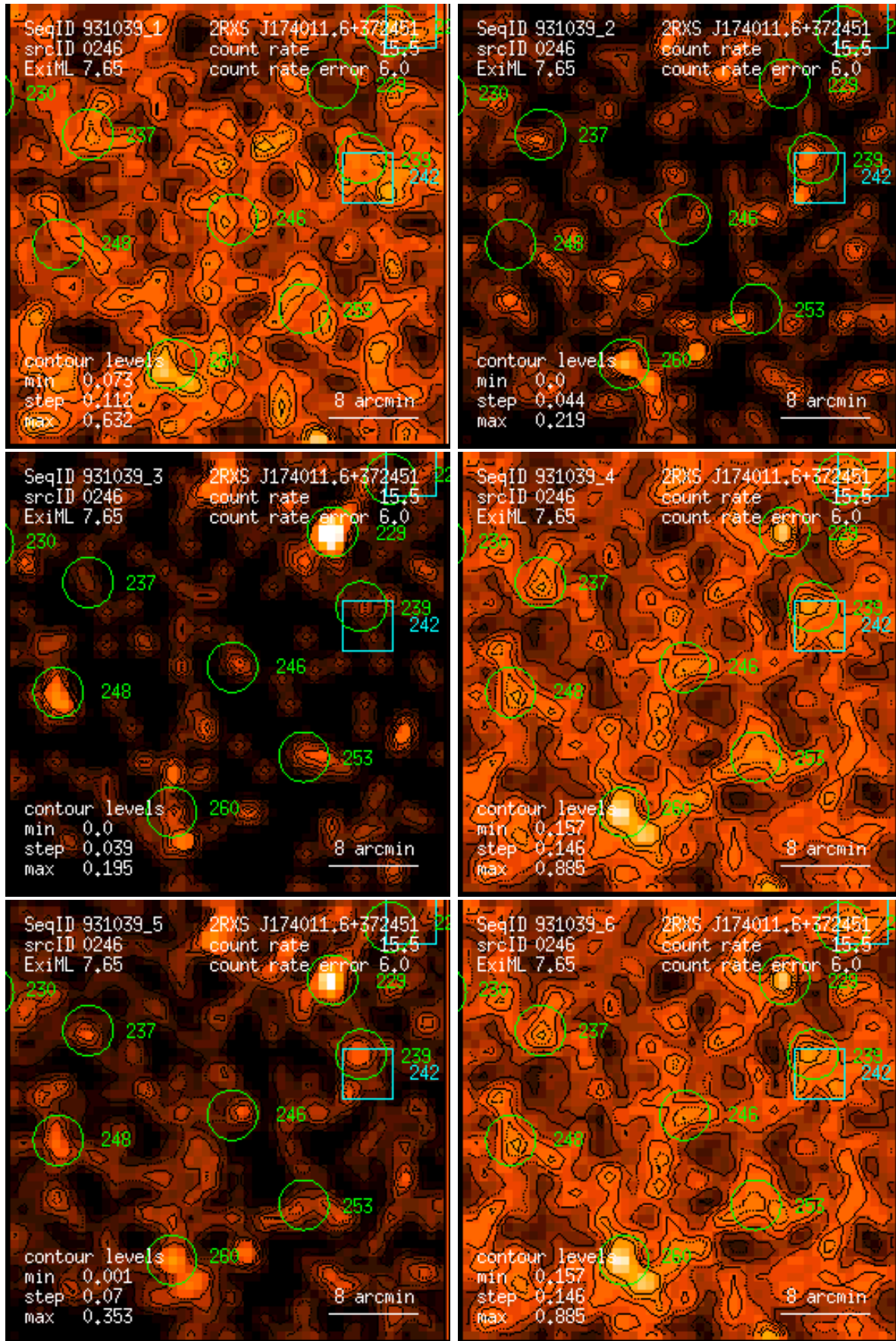
Figure 246: RASS 931039: detection 0246: band rate images, Gaussian filter: (1) PSPC channels 11 – 41, (2) 52 – 90, (3) 91 – 201, (4) 11 – 235, (5) 52 – 201, (6) 11 – 201. Broad band rates in counts/ks. Band rate contour levels in counts/ks/arcmin 2 .
