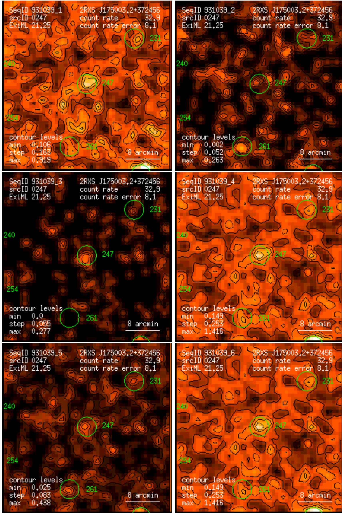
Figure 247: RASS 931039: detection 0247: band rate images, Gaussian filter: (1) PSPC channels 11 – 41, (2) 52 – 90, (3) 91 – 201, (4) 11 – 235, (5) 52 – 201, (6) 11 – 201. Broad band rates in counts/ks. Band rate contour levels in counts/ks/arcmin 2 .
