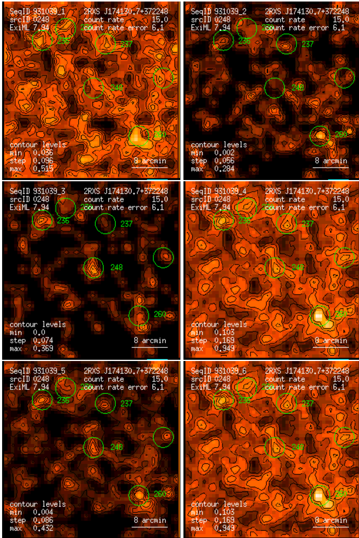
Figure 248: RASS 931039: detection 0248: band rate images, Gaussian filter: (1) PSPC channels 11 – 41, (2) 52 – 90, (3) 91 – 201, (4) 11 – 235, (5) 52 – 201, (6) 11 – 201. Broad band rates in counts/ks. Band rate contour levels in counts/ks/arcmin 2 .
