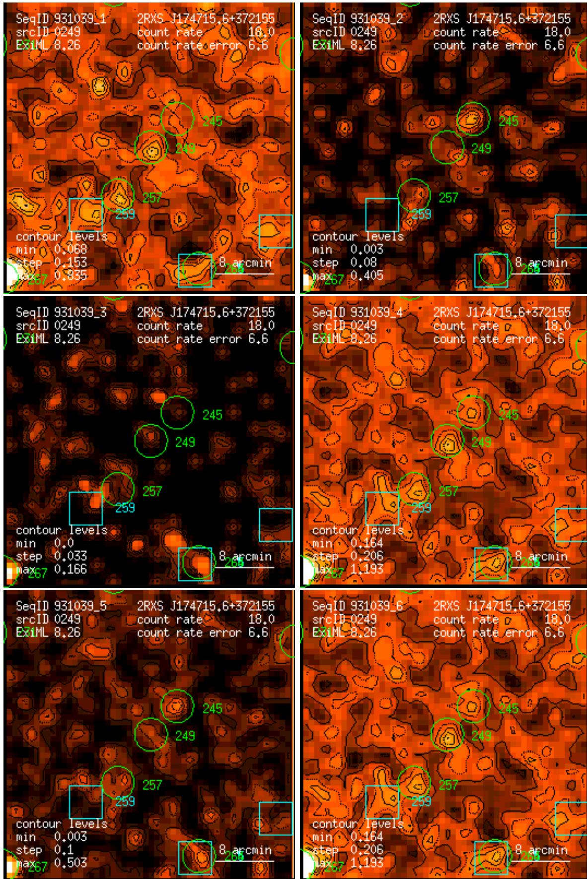
Figure 249: RASS 931039: detection 0249: band rate images, Gaussian filter: (1) PSPC channels 11 – 41, (2) 52 – 90, (3) 91 – 201, (4) 11 – 235, (5) 52 – 201, (6) 11 – 201. Broad band rates in counts/ks. Band rate contour levels in counts/ks/arcmin 2 .
