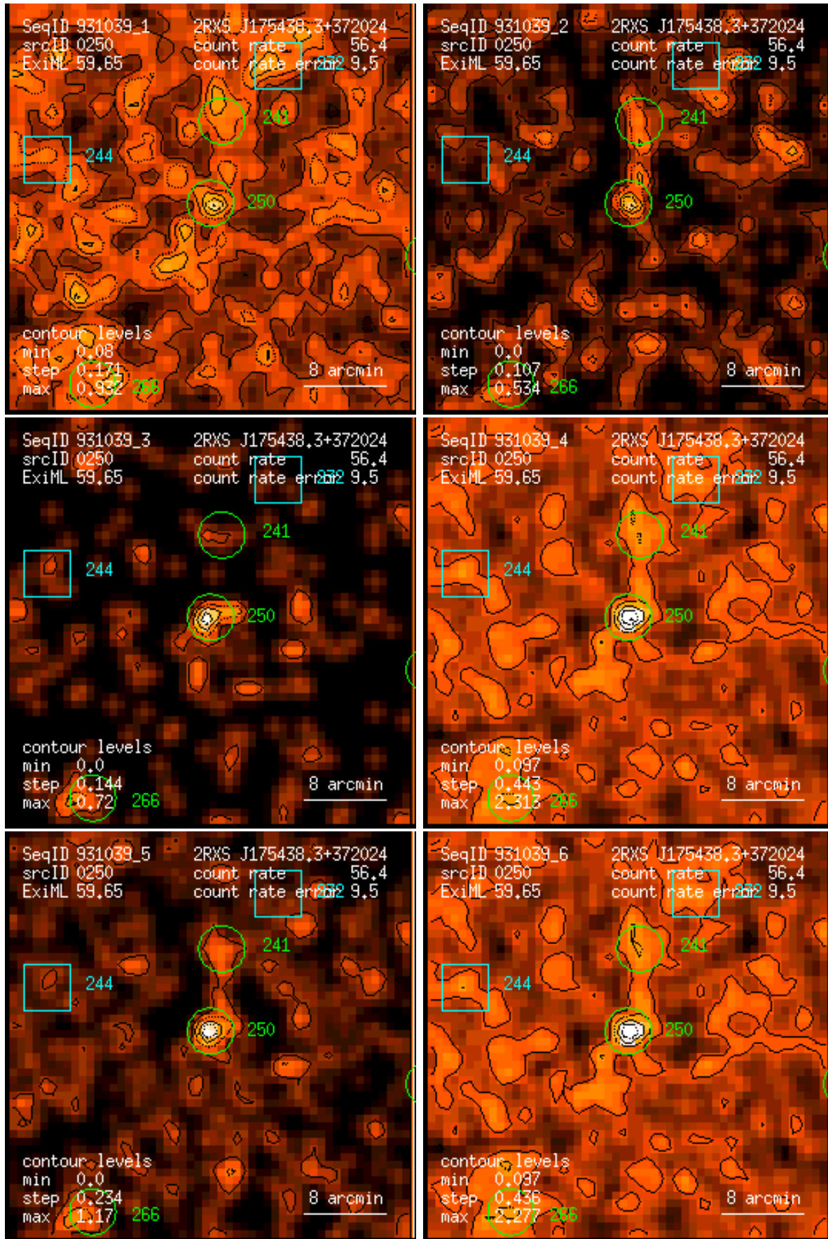
Figure 250: RASS 931039: detection 0250: band rate images, Gaussian filter: (1) PSPC channels 11 – 41, (2) 52 – 90, (3) 91 – 201, (4) 11 – 235, (5) 52 – 201, (6) 11 – 201. Broad band rates in counts/ks. Band rate contour levels in counts/ks/arcmin 2 .
