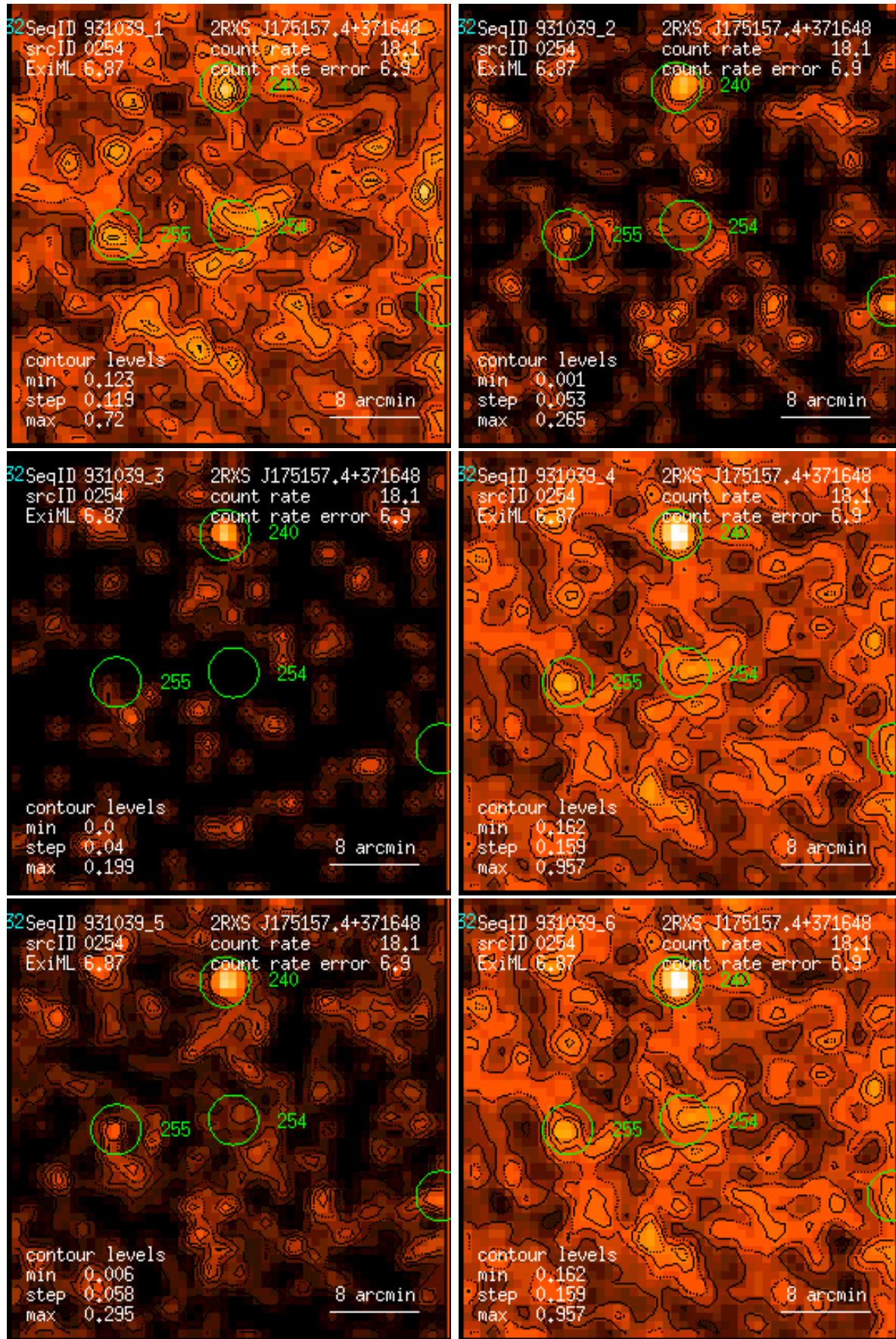
Figure 254: RASS 931039: detection 0254: band rate images, Gaussian filter: (1) PSPC channels 11 – 41, (2) 52 – 90, (3) 91 – 201, (4) 11 – 235, (5) 52 – 201, (6) 11 – 201. Broad band rates in counts/ks. Band rate contour levels in counts/ks/arcmin 2 .
