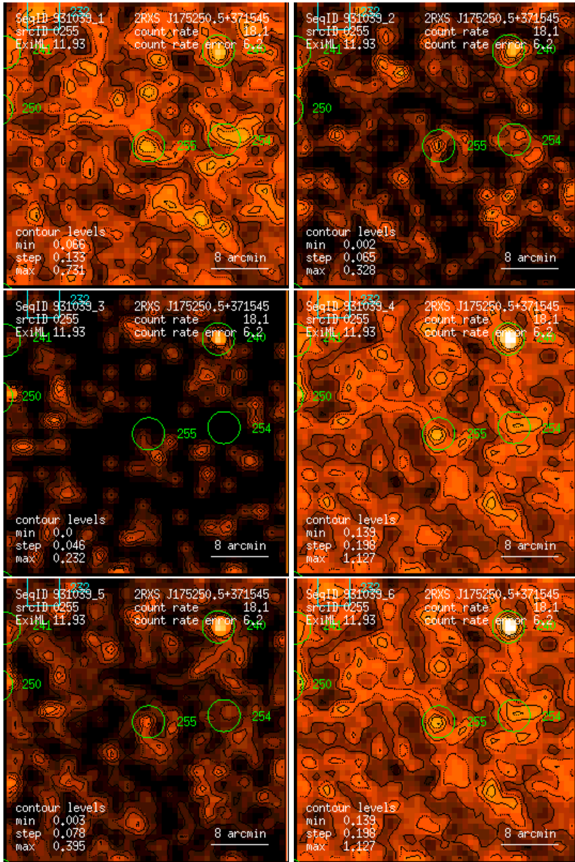
Figure 255: RASS 931039: detection 0255: band rate images, Gaussian filter: (1) PSPC channels 11 – 41, (2) 52 – 90, (3) 91 – 201, (4) 11 – 235, (5) 52 – 201, (6) 11 – 201. Broad band rates in counts/ks. Band rate contour levels in counts/ks/arcmin 2 .
