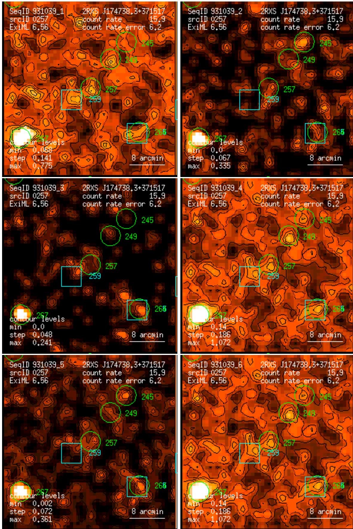
Figure 257: RASS 931039: detection 0257: band rate images, Gaussian filter: (1) PSPC channels 11 – 41, (2) 52 – 90, (3) 91 – 201, (4) 11 – 235, (5) 52 – 201, (6) 11 – 201. Broad band rates in counts/ks. Band rate contour levels in counts/ks/arcmin 2 .
